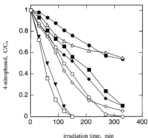
Figure 9. Photooxidation of 4-nitrophenol in the presence of TiO 2 and of various samples containing 1% of transition metal. Symbols are the same as in Figure 5.
