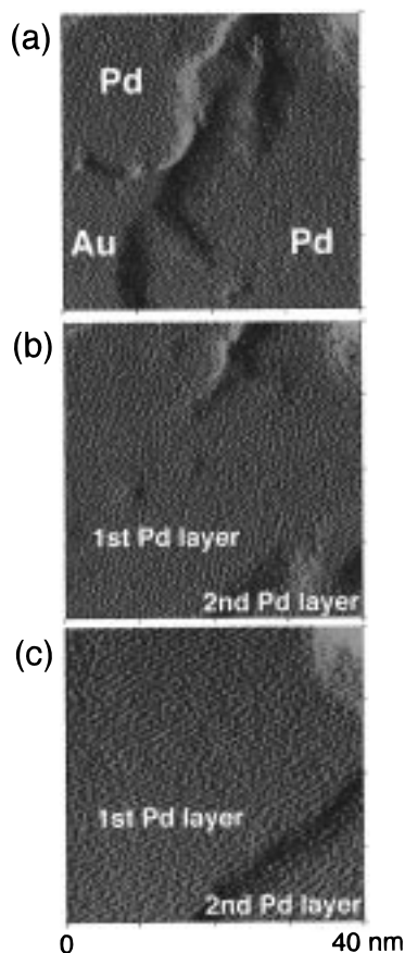
Figure 7. Sequentially obtained higher resolution STM images ( 40 \times 40 \text{ nm}^2 ) of the palladium deposition process on an Au(111) substrate (a) 20 s, (b) 40 s, and 2 min after the potential was stepped from +0.95 to +0.87 V in 50 mM \text{H}_2\text{SO}_4 solution containing 0.5 mM \text{PdCl}_4^{2-} .
