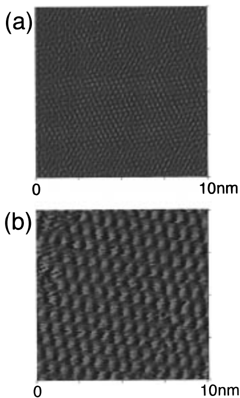
Figure 2. STM images ( 10 \times 10 \text{ nm}^2 ) of (a) an Au(111)– (1 \times 1) electrode obtained at +0.95 V in a 50 mM \text{H}_2\text{SO}_4 solution and (b) the same electrode in a 50 mM \text{H}_2\text{SO}_4 solution containing 0.1 mM \text{PdCl}_4^{2-} while the electrode potential was kept constant at +0.95 V.
