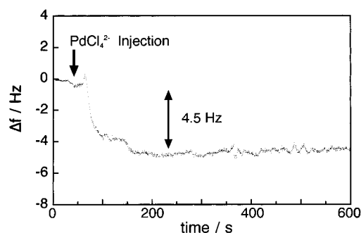
Figure 1. Time dependence of frequency change at +0.95 V when the \text{PdCl}_4^{2-} solution was added to the EQCM cell that contained a 50 mM \text{H}_2\text{SO}_4 solution. The final concentration of \text{PdCl}_4^{2-} in the cell was 0.1 mM.
