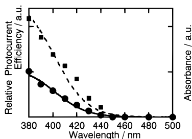
Figure 13. Action spectra of composite films and absorption spectra of CdS-nanoparticle dispersion before being immobilized. Circles and squares correspond to the relative photocurrent efficiency of Au-dt-CdS and Au-dt-CdS-dt-CdS, respectively, and solid and dashed lines show the absorption spectrum on different scales.
