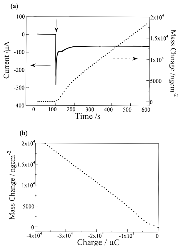
Figure 2. (a) Time dependence of current (solid line) and the mass change (dotted line) at a gold/EQCM electrode in a solution containing 50 mM \text{HClO}_4 and 0.6 mM \text{H}_2\text{PtCl}_6 when the potential was stepped from +1.0 to +0.60 V, as shown by the arrow. (b) Relationship between the mass change and electric charge after the potential was stepped from +1.0 to +0.60 V, shown in part a.
