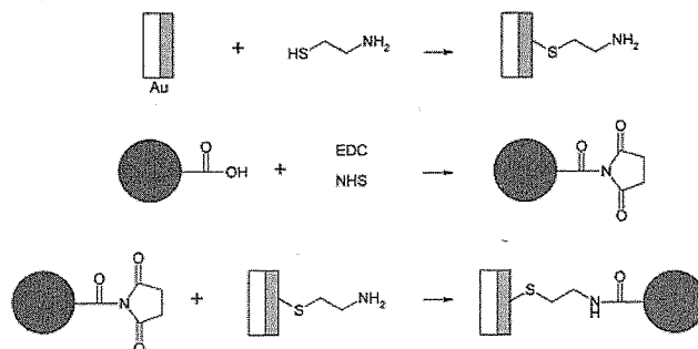
Figure 18. Schematic modification process of fluorescent nanospheres containing a large number ( \sim 10^6 per sphere) of pendant carboxylic acid moieties, which were exploited to couple the nanospheres to amine-terminated thiol SAMs through amide bond formation. Reprinted with permission from [142], S. T. Plummer and P. W. Bohn, Langmuir 18, 4142 (2002). © 2002, American Chemical Society.
