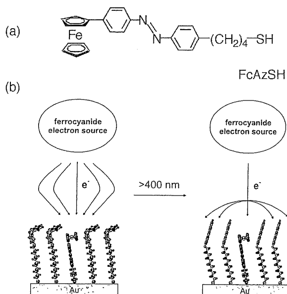
Figure 11. (a) FcAzSH molecule. (b) Schematic illustration of the control of electron transfer by photo-irradiation at FcAzSH SAM-modified gold electrodes. Reprinted with permission from [113], D. G. Walter et al., J. Phys. Chem. B 103, 402 (1999). © 1999, American Chemical Society.
