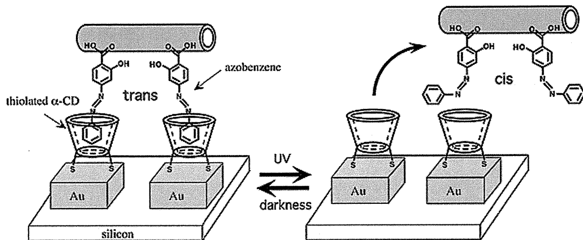
Figure 17. Schematic diagram of an azobenzene nanotube assembly on complementary \alpha -CD SAM/Au substrates via host-guest molecular recognition and light-induced nanotube detachment/attachment on the \alpha -CD SAM surface. Reprinted with permission from [138], I. A. Banerjee et al., J. Am. Chem. Soc. 125, 9542 (2003). © 2003, American Chemical Society.
