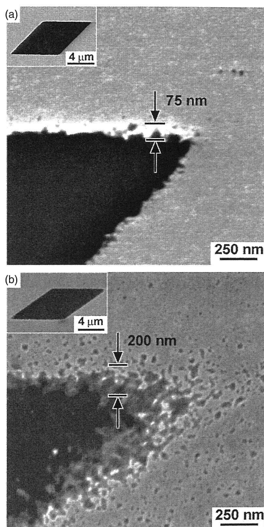
Figure 25. (a) SEM of a diamond pattern on Pd. The pattern was generated by two consecutive printings of 5-μm lines (10-μm pitch) at an angle of ~30° relative to one another. The edge roughness is ~30–70 nm and the radius of curvature at the point of the structure is ~40–50 nm. The inset shows the whole diamond. (b) SEM of a diamond pattern of gold. Note the increase in the number of pits in the surface of the gold and the radius of curvature in the point (~150 nm). Reprinted with permission from [161], J. C. Love et al., J. Am. Chem. Soc. 124, 1576 (2002), © 2002, American Chemical Society.
