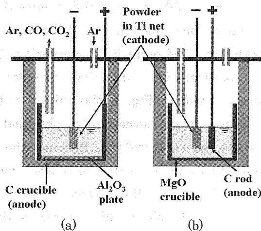
Fig. 2 Experimental setups. (a) a wide anodic area is obtained by carbon crucible, and (b) the closer electrode distance can be set.
