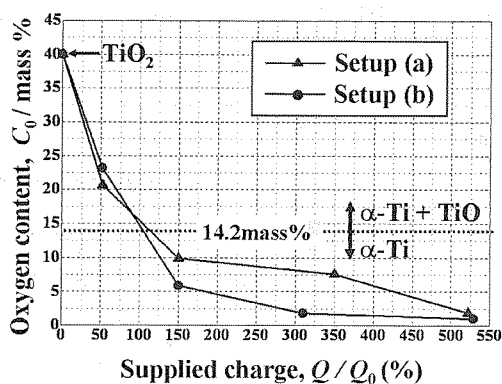
Fig. 3 Oxygen concentration in the samples. The supplied electricity Q is normalized by Q_0 , the theoretical electricity to form the necessary amount of Ca for the reduction. The Ti-O solid solution can be obtained below 14.2% at 1173 K according to the phase diagram[21].
