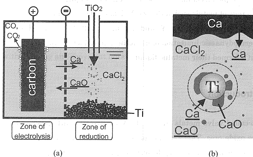
Fig.1 (a) Concept of OS process and (b) removal of CaO into molten \text{CaCl}_2 .
