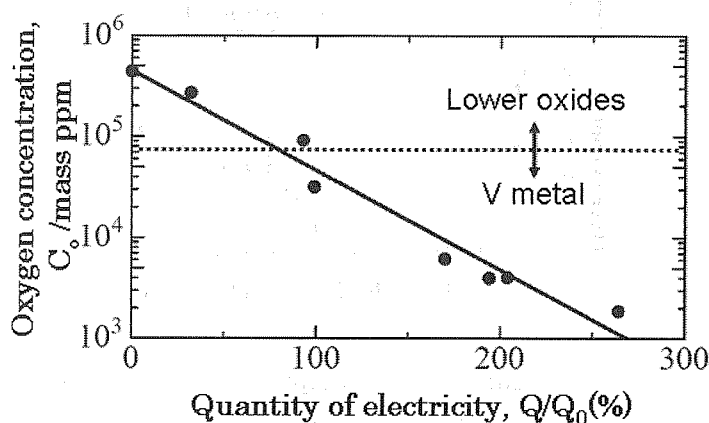
Fig. 4 Oxygen concentration in the obtained samples. The V-O solid solution was obtained below 7 mass% at 1173 K, which corresponded to the phase diagram[21].
