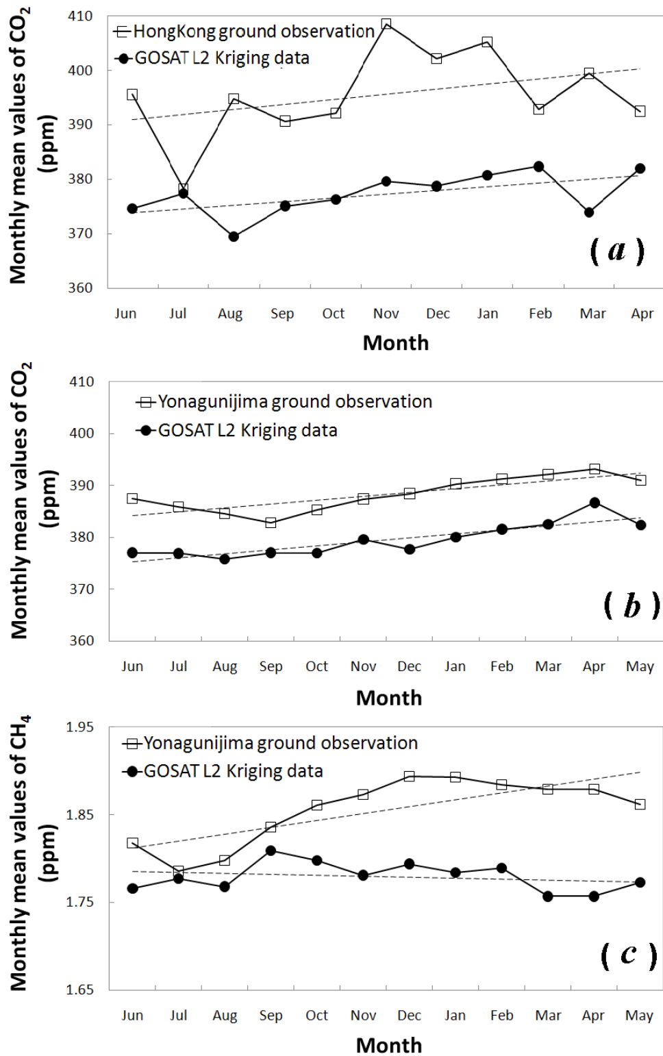
Figure 12. Monthly mean values of the Level 2 Kriging interpolation data and ground observation data: (a) \text{XCO}_2 in the Hong Kong site, (b) \text{XCO}_2 in the Yonaguni-jima site in Japan and (c) \text{XCH}_4 in the Yonaguni-jima site in Japan.
