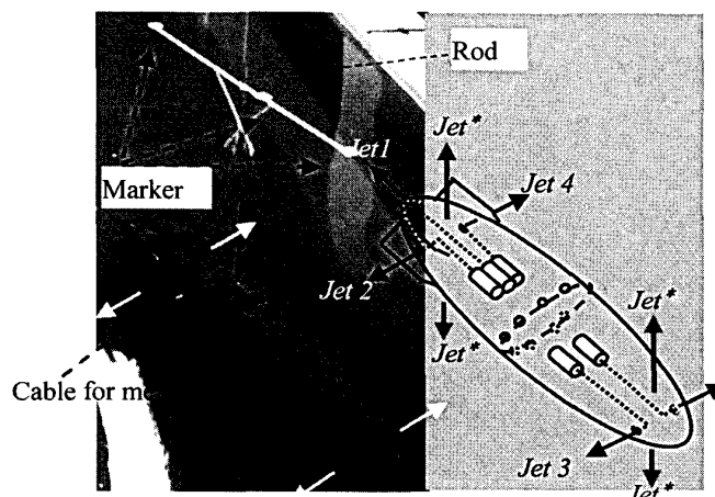
Fig.13 Photograph of model and arrangement of water-jet pumps and position markers.
