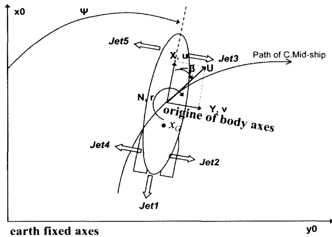
Fig.3 Coordinate systems.
