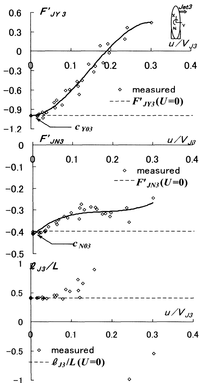
Fig.6 Non-dimensional lateral force and yaw moment for various ship's velocity ratio by Jet 3.
