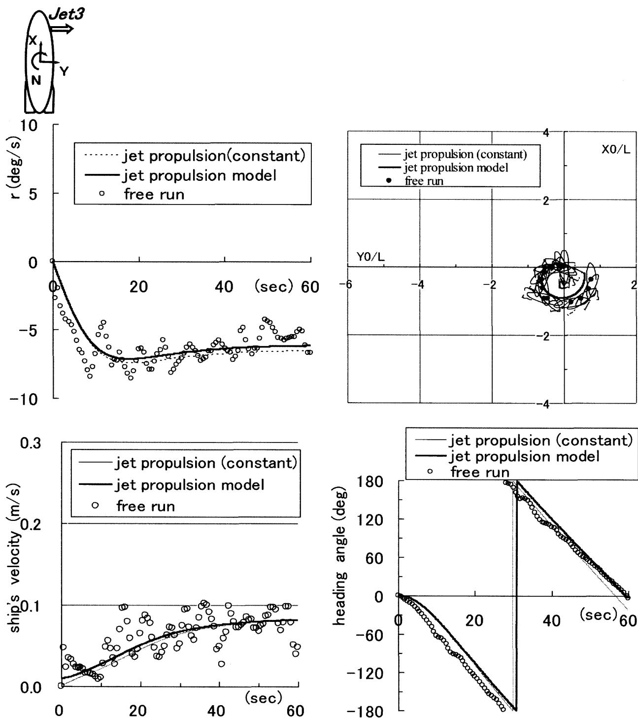
Fig.15 Comparison of trajectory, ship's velocity, r and heading angle by Jet 3 between measured and simulated.
