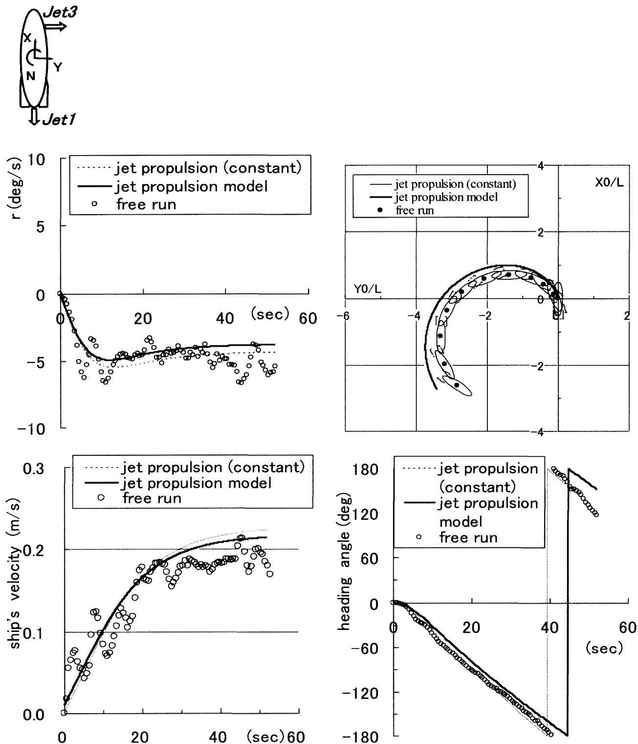
Fig.14 Comparison of trajectory, ship's velocity, r and heading angle by Jet 1 and Jet 3 between measured and simulated.
