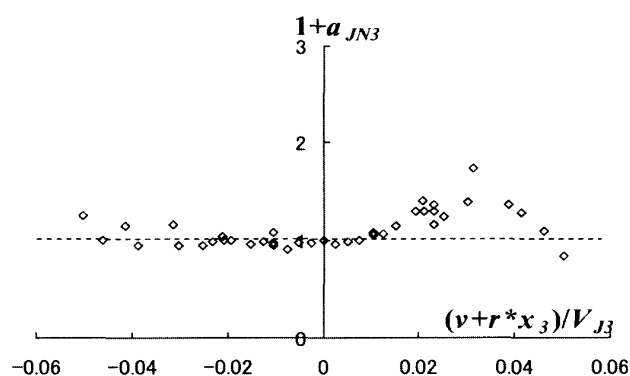
Fig.8 (1+a_{JY}) and (1+a_{JN}) of jet 3.
