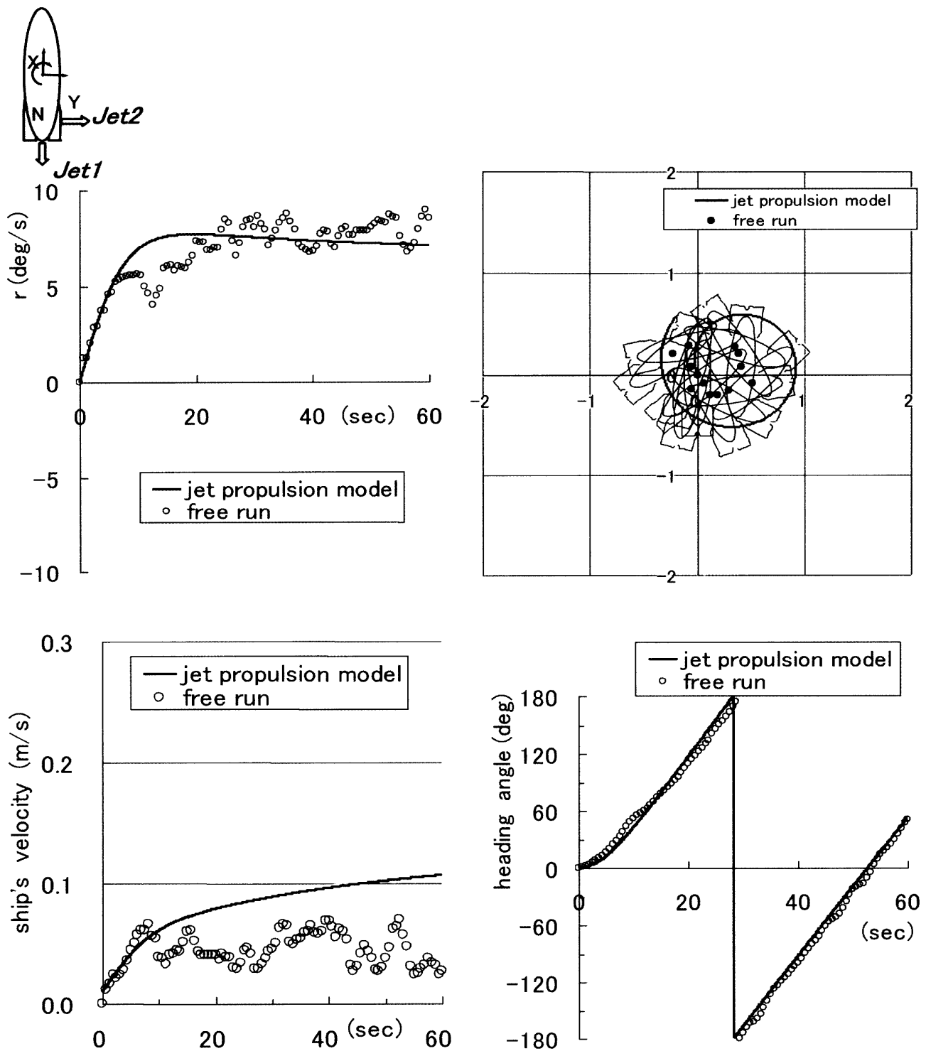
Fig.16 Comparison of trajectory, ship's velocity, r and heading angle by Jet 1 and Jet 2 between measured and simulated.
