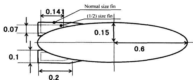
Fig.5 Side view. (unit : meter)
