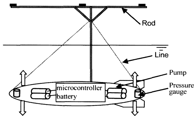
Fig.12 Vertical control system for free run tests.
