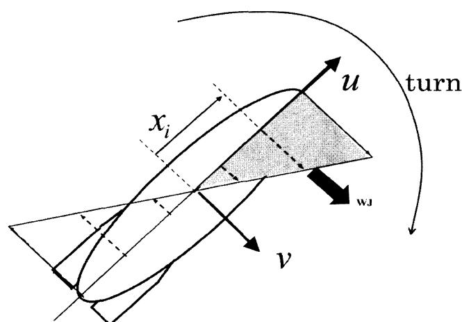
Fig.7 Lateral velocity v_i on the outlet of Jet.
