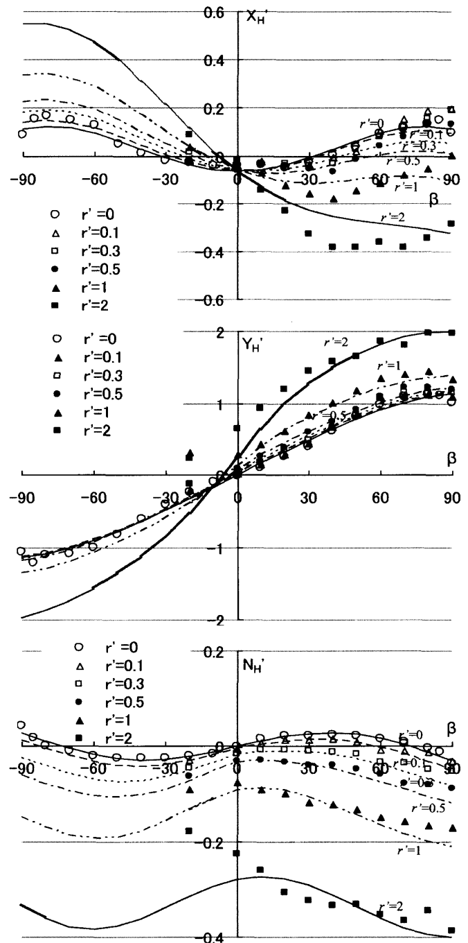
Fig.4 Comparison of hull force components between measured and approximated (with normal size fin).
