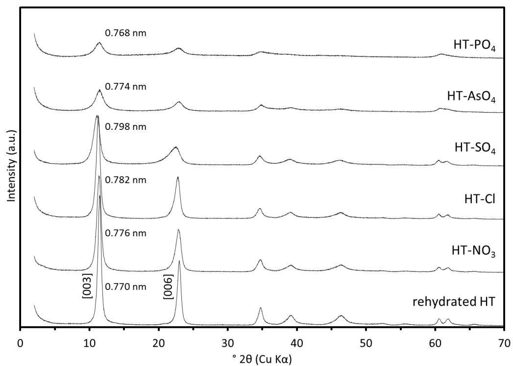
Fig. 2. XRD patterns of rehydrated HT and HT with different anions. The initial anion concentration was adjusted to 10 mmol/L for each sample.
