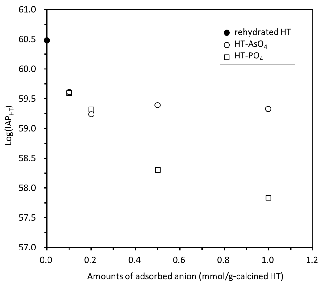
Fig. 6. IAP_{HT} in the reacted solutions as a function of the amount of adsorbed anions.
