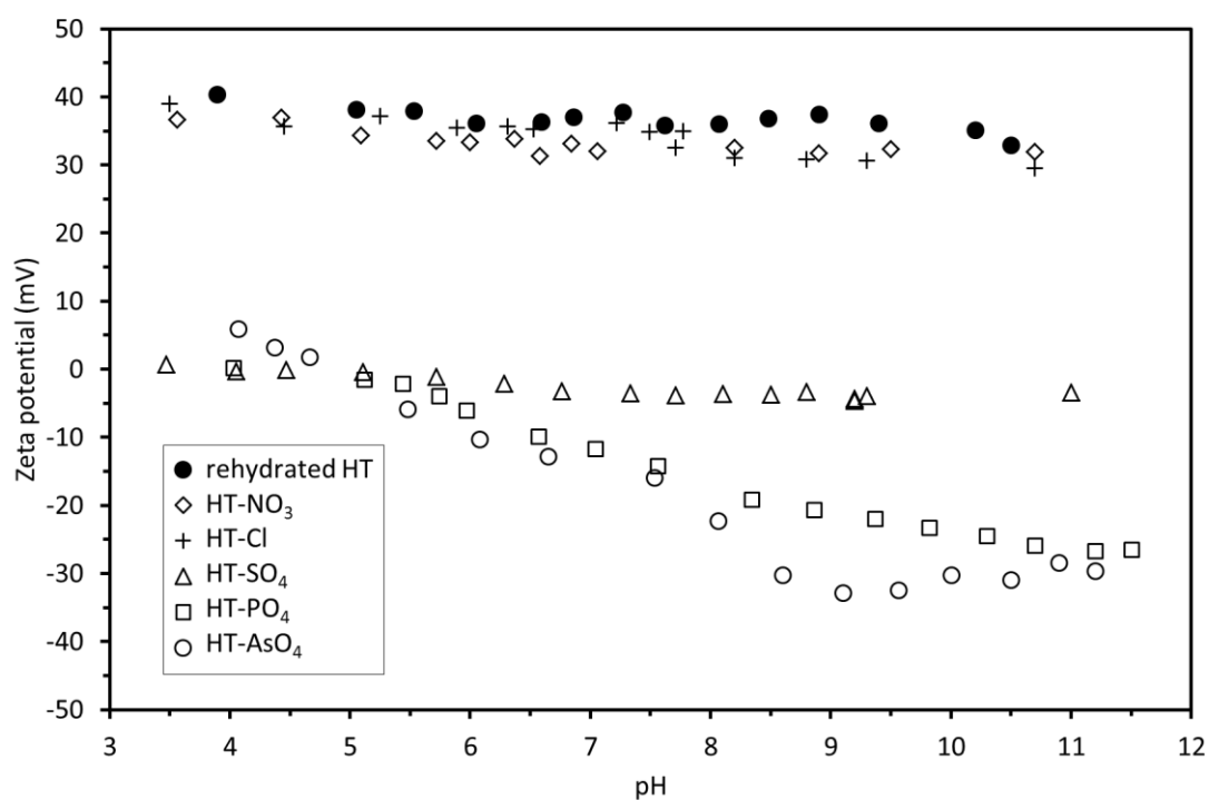
Fig. 5. Changes in the zeta potential of rehydrated HT and HT with the different anions as a function of pH. The initial anion concentration was adjusted to 10 mmol/L for each sample. The concentrations of suspended solids were adjusted to 1.0 g/L, and a pH was changed by adding 0.1 mol/L HNO 3 solution.
