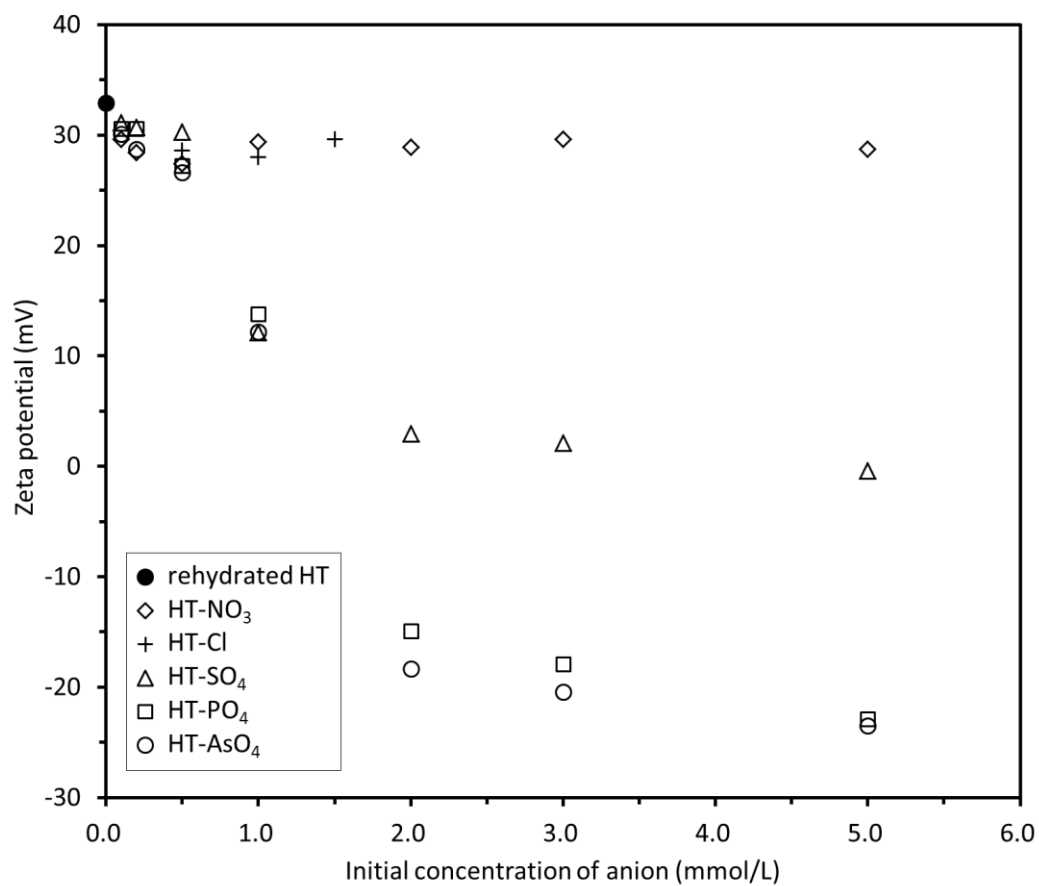
Fig. 3. Zeta potentials of HT with the different anions. The equilibrium pH of rehydrated HT suspension was 10.6. The equilibrium pH ranged from 10.7 to 11.1 in the NO 3 system, from 10.8 to 10.9 in the Cl system, from 10.8 to 11.4 in the SO 4 system, from 10.7 to 11.3 in the AsO 4 system, and from 10.6 to 11.4 in the PO 4 system.
