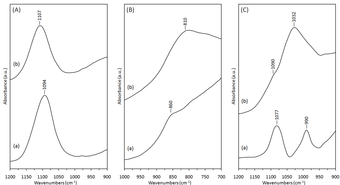
Fig. 4. (A) ATR-FTIR spectra of SO 4 : (a) the 0.5 mol/L Na 2 SO 4 solution adjusted to pH 10, and (b) HT-SO 4 with 0.865 mmol-SO 4 /g-calcined HT. (B) ATR-FTIR spectra of AsO 4 : (a) the 0.5 mol/L Na 2 HAsO 4 solution adjusted to pH 10, and (b) HT-AsO 4 with 1.91 mmol-AsO 4 /g-calcined HT. (C) ATR-FTIR spectra of PO 4 : (a) the 0.5 mol/L Na 2 HPO 4 solution adjusted to pH 10, and (b) HT-PO 4 with 2.11 mmol-PO 4 /g-calcined HT.
