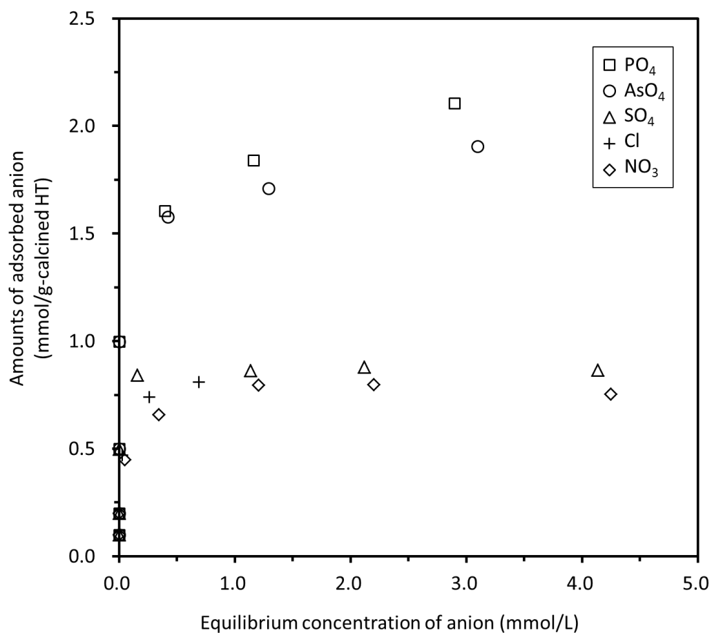
Fig. 1. Adsorption isotherms for the anions onto HT. Equilibrium pH ranged from 10.7 to 11.1 in the NO 3 system, from 10.8 to 10.9 in the Cl system, from 10.8 to 11.4 in the SO 4 system, from 10.7 to 11.3 in the AsO 4 system, and from 10.6 to 11.4 in the PO 4 system. The concentrations of solids were adjusted to 1.0 g/L. Each plot indicates the average of two different samples.
