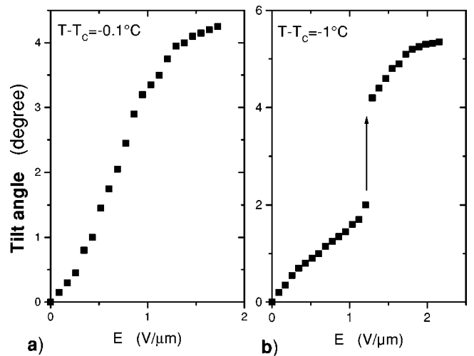
FIG. 3. Apparent tilt angle variation under dc field at (a) T - T_C = -0.1\ ^\circ\text{C} , (b) T - T_C = -1\ ^\circ\text{C} .
