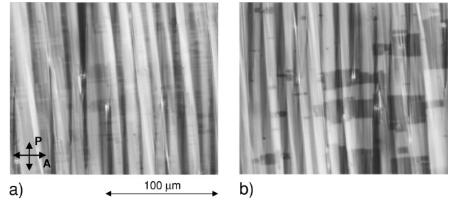
FIG. 2. The microphotographs of the texture in the \text{SmC}_\alpha^* phase under a dc electric field at (a) T - T_C = -0.6\ ^\circ\text{C} , E = 1.15\ \text{V}/\mu\text{m} ; (b) T - T_C = -1.0\ ^\circ\text{C} , E = 1.25\ \text{V}/\mu\text{m} . The polarizers are crossed.
