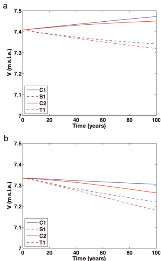
Fig. 9. Ice volume ( V ) changes simulated with (a) Elmer/Ice and (b) SICOPOLIS for experiments C1 (constant climate control run), S1 (constant climate forcing, doubled basal sliding), C2 (AR4 climate forcing) and T1 (AR4 climate forcing, doubled basal sliding). Note that t = 0 corresponds to the year 2004.
