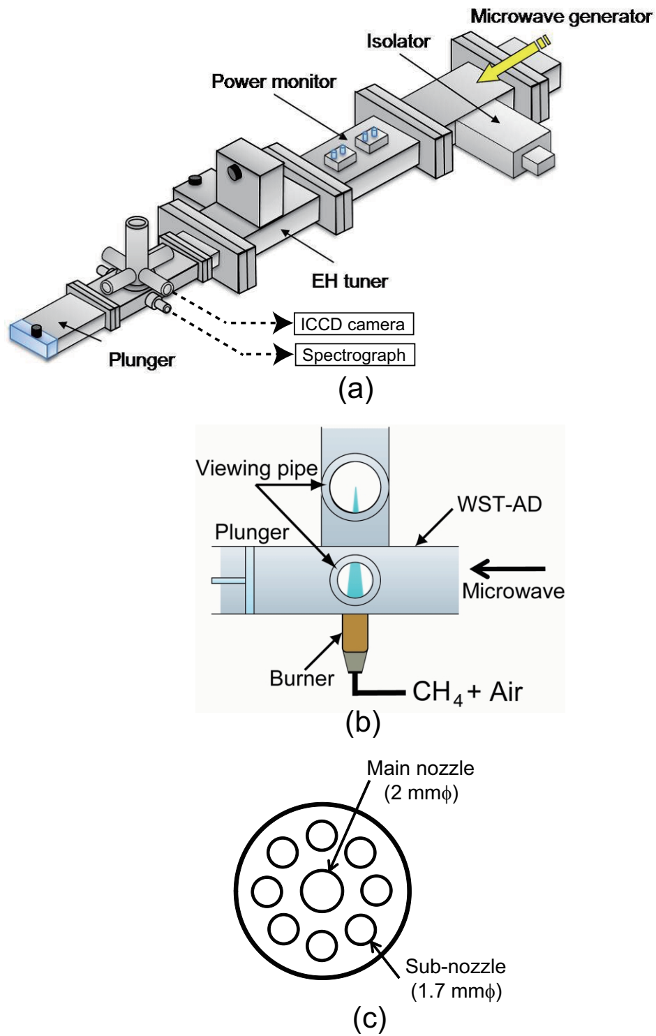
Figure 1. Schematic illustrations of experimental apparatus. (a) Transmission system for microwave, (b) an enlarged illustration of microwave-irradiation part, and (c) the structure of the nozzles.
