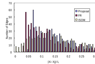
図7 エッジ長の度数分布(College football) Fig.7 Histogram of edge length (College football)
