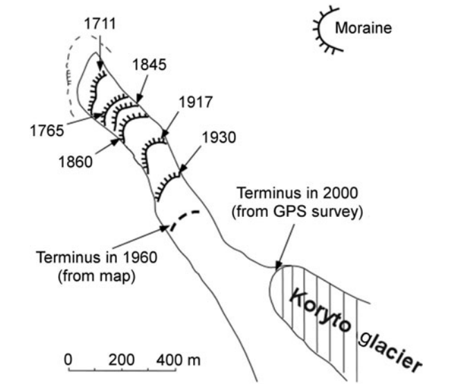
Fig. 3. Distribution of terminal moraines at Koryto glacier, modified from Solomina (1999) using the GPS data surveyed in 2000.
