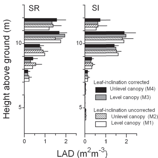
Fig. 5. LAD profiles generated by the four models (M1–M4 in Section 2.8). In the unlevel canopy models (M2 and M4), standard errors among the 10 measurement sites are given by horizontal line segments.
