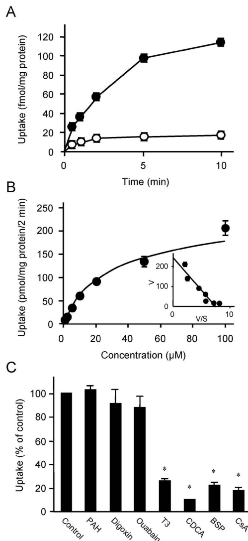
Fig. 2. Characteristics of estrone 3-sulfate transport by OATP4C1
