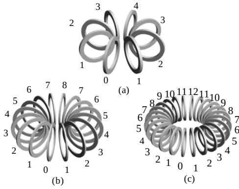
Fig. 2. The external view of the m -toroidal SMES coils with numbering the superconducting element coils. (a) 8-toroidal magnet, (b) 16-toroidal magnet, and (c) 24-toroidal magnet.
