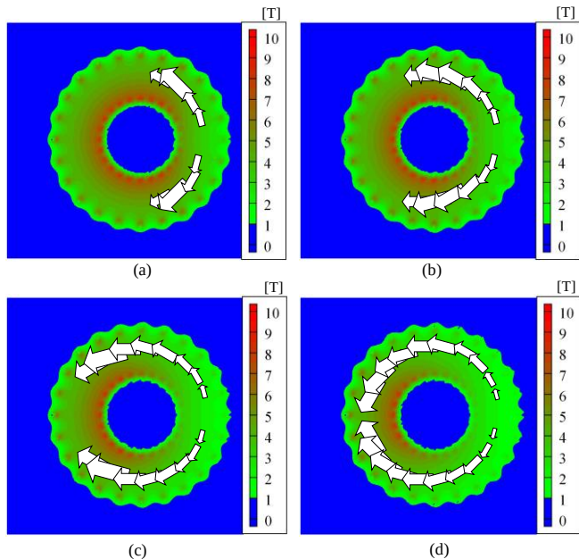
Fig. 9. The distribution of the magnetic field when the overturning force on (a) the 3rd, (b) 5th, (c) 7th, and (d) 9th superconducting element coil of 24-toroidal HTS-SMES magnet reaches to its peak, respectively. The arrows denote the overturning force on superconducting element coils.
