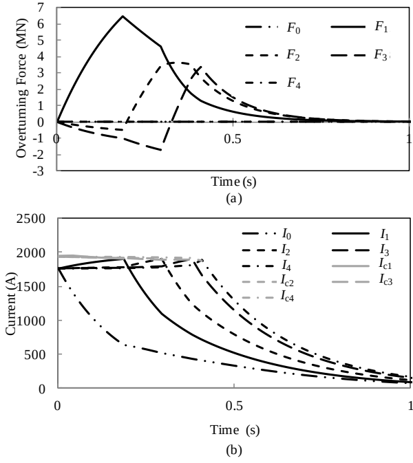
Fig. 5. The time transitions of (a) the overturning force F_k , (b) the coil current I_k and critical current I_{ck} of 8-toroidal HTS-SMES magnet during the chain of quenches after the 0th superconducting element coil transitions into the normal state at t = 0 .
