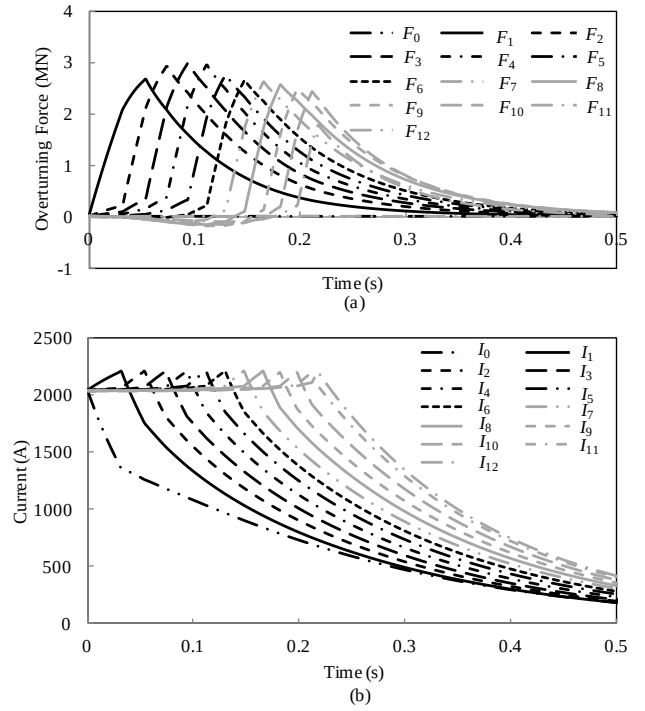
Fig. 7. The time transitions of (a) the overturning force F_k , (b) the coil current I_k and critical current I_{ck} of 24-toroidal HTS-SMES magnet during the chain of quenches after the 0th superconducting element coil transitions into the normal state at t = 0 .
