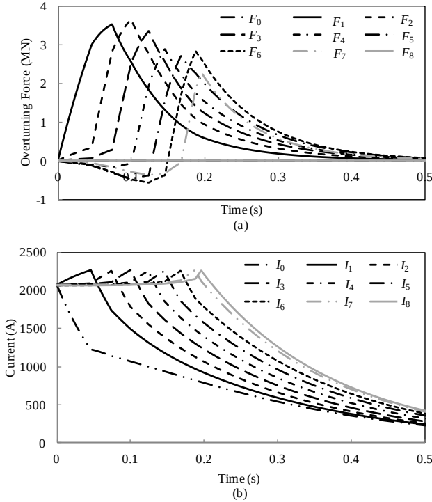
Fig. 6. The time transitions of (a) the overturning force F_k , (b) the coil current I_k and critical current I_{ck} of 16-toroidal HTS-SMES magnet during the chain of quenches after the 0th superconducting element coil transitions into the normal state at t = 0 .
