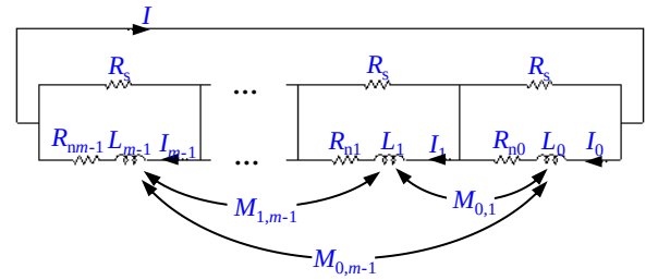
Fig. 3. The electrical circuit of the m -toroidal HTS-SMES system with the shunt resistors.
