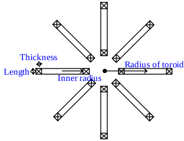
Fig. 1. The schematic view of 8-toroidal HTS-SMES magnet with design variables, where are the inner radius, the length, the thickness, and the radius of toroid.
