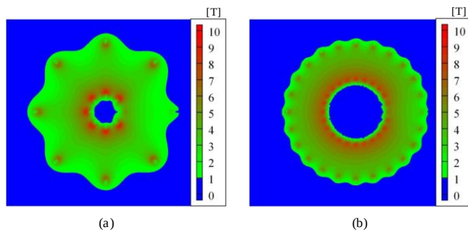
Fig. 8. The distribution of the magnetic field when the overturning force on the 1st superconducting element coil reaches to its peak. (a) 8-toroidal and (b) 24-toroidal HTS-SMES magnet.
