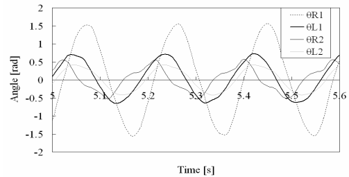
Fig. 3 Flapping and feathering angles for the best creature
