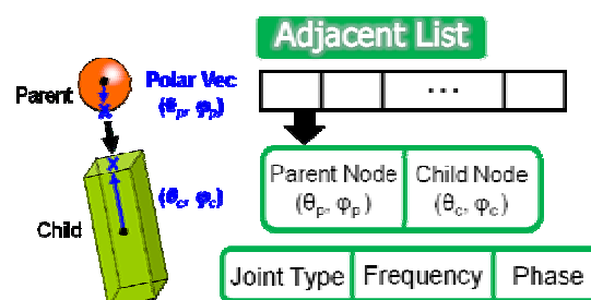
Fig.2 Adjacent List
