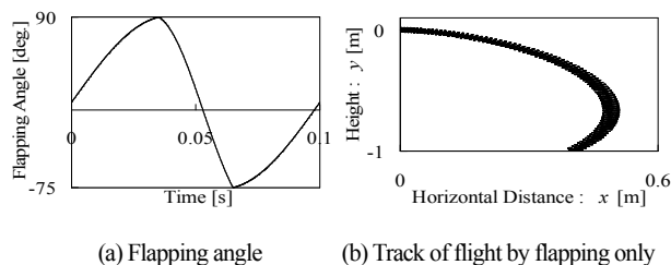
Fig. 3 Flapping angle and track of flight
