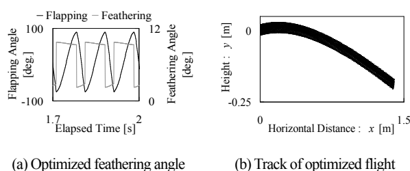
Fig. 4 Optimized feathering angle and track of flight
