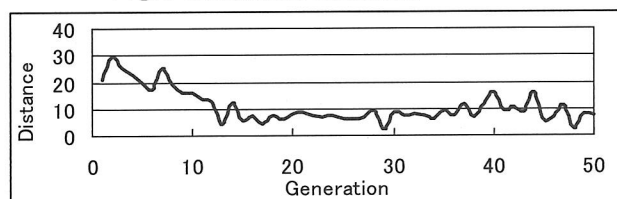
Fig. 6 Distance between model and light source
