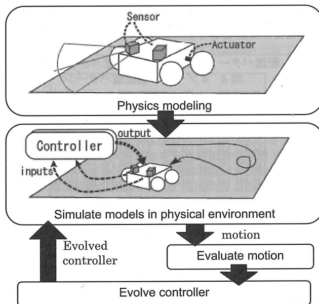
Fig. 1 Software architecture
