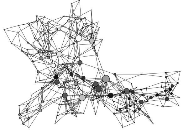
図 2 A network colored in characteristic frequency ( \sigma = 1.0 )
