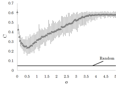
図 3 Variation of C vs \sigma
