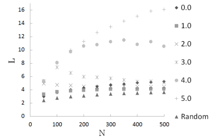
図 5 Variation of L vs N
