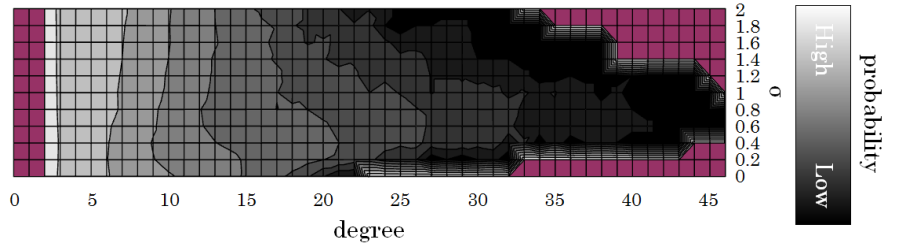
図 7 Variation of degree distribution with \sigma
