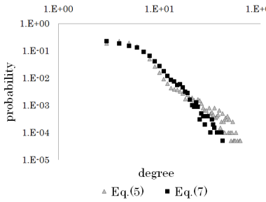
図 6 Degree distribution ( \sigma = 1.0 )
