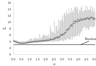
図 4 Variation of L vs \sigma
