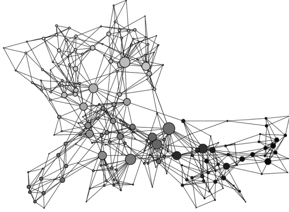
図 1 A network colored in frequency ( \sigma = 1.0 )
