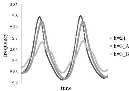
図 8 Variation of frequency vs elapsed time in degree
