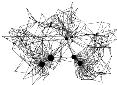
図 11 Obtained network using condition I
