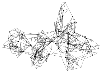
図 12 Obtained network using condition II
