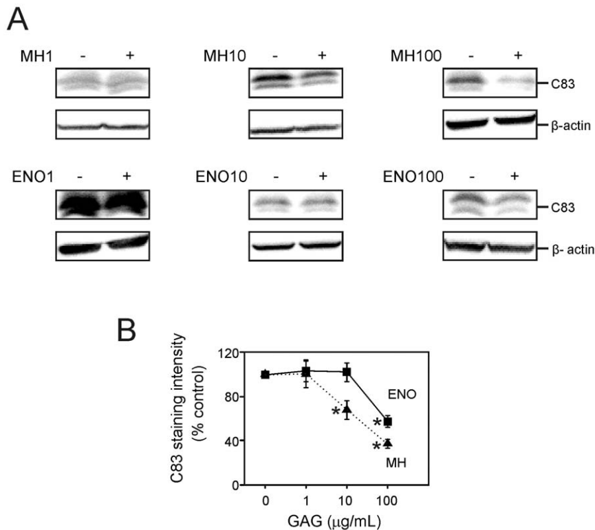
Figure 5. Effects of heparin and enoxaparin in the presence of 0.5 \mu M DAPT on C83 in Tg2576 mouse cortical cells. (A) Cells were incubated in the presence or absence of 1, 10 or 100 \mu g/mL heparin (MH1, MH10 or MH100, respectively) or 1, 10 or 100 \mu g/ml enoxaparin (ENO1, ENO10 or ENO100, respectively) for 24 hours. Cell lysates were then analysed by western blotting using polyclonal anti-APP C-terminal antibody to determine the level of C83. The level of \beta -actin immunoreactivity was used as a loading control. (B) Quantification of the level of C83 immunoreactivity. Asterisks show values that are significantly different from controls ( p < 0.001 , n = 9 ). doi:10.1371/journal.pone.0023007.g005
