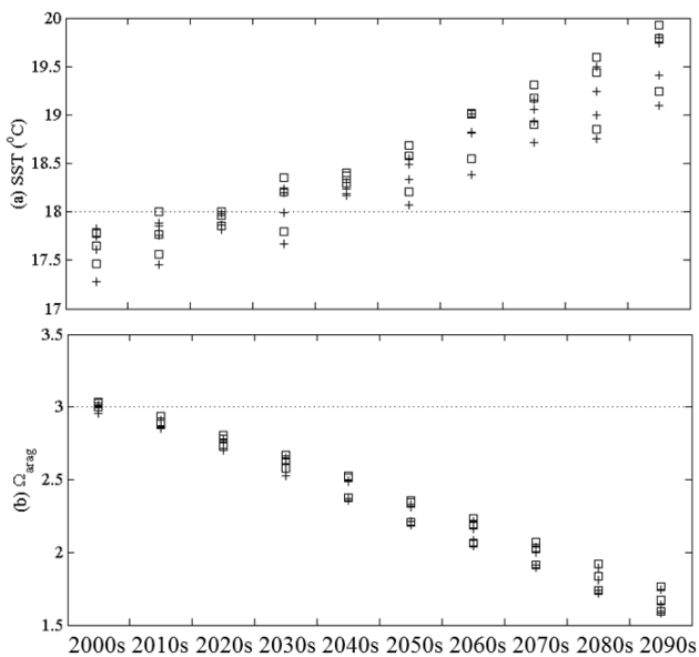
Fig. 6. Decadal-mean (a) SST ( ^{\circ}\text{C} ) during the coldest months and (b) annual lowest \Omega_{\text{arag}} (2000s–2090s) at Kushimoto-Shirahama ( 135.7^{\circ}\text{E} , 33.5^{\circ}\text{N} ) and Tateyama ( 139.8^{\circ}\text{E} , 35.0^{\circ}\text{N} ) projected by the four climate models. Squares denote the projected SST and \Omega_{\text{arag}} at Kushimoto-Shirahama. Crosses show the projected SST and \Omega_{\text{arag}} at Tateyama. A dotted line in (a) and (b) denotes a SST = 18^{\circ}\text{C} and \Omega_{\text{arag}} = 3 line, respectively.
