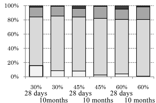
Fig. 2 Volume ratio of microscopic geometrical model
