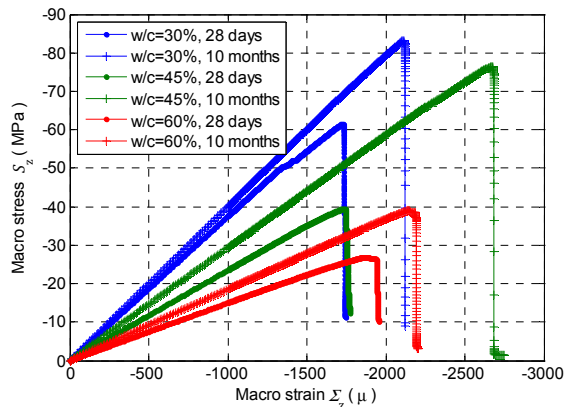
Fig. 15 Difference in w/c and age ( G_f = 10^{-5} N/mm, \varepsilon_u = 500\mu )
