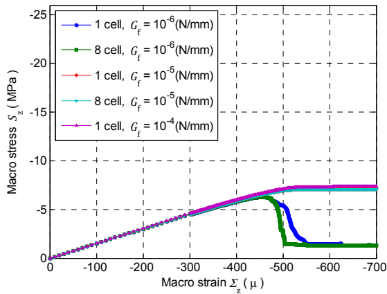
Fig. 8 Influence of periodic boundary and fracture energy (w/c=60%, Age=28 days)
