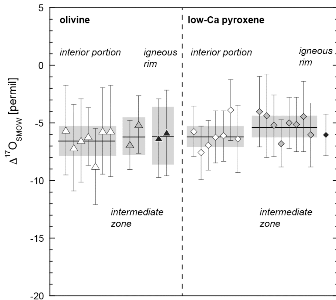
1 Fig. 9 The oxygen isotopic compositions of olivines and low-Ca in the interior portion, 2 the igneous rim and the intermediate zone are compared by \Delta^{17}\text{O} value. The horizontal 3 lines and gray areas are the weighted average and 2 sigma errors for each mineral and 4 area, respectively. The ^{16}\text{O} -enrichment of olivines and low-Ca pyroxenes in all three 5 areas is essentially identical within analytical error.
