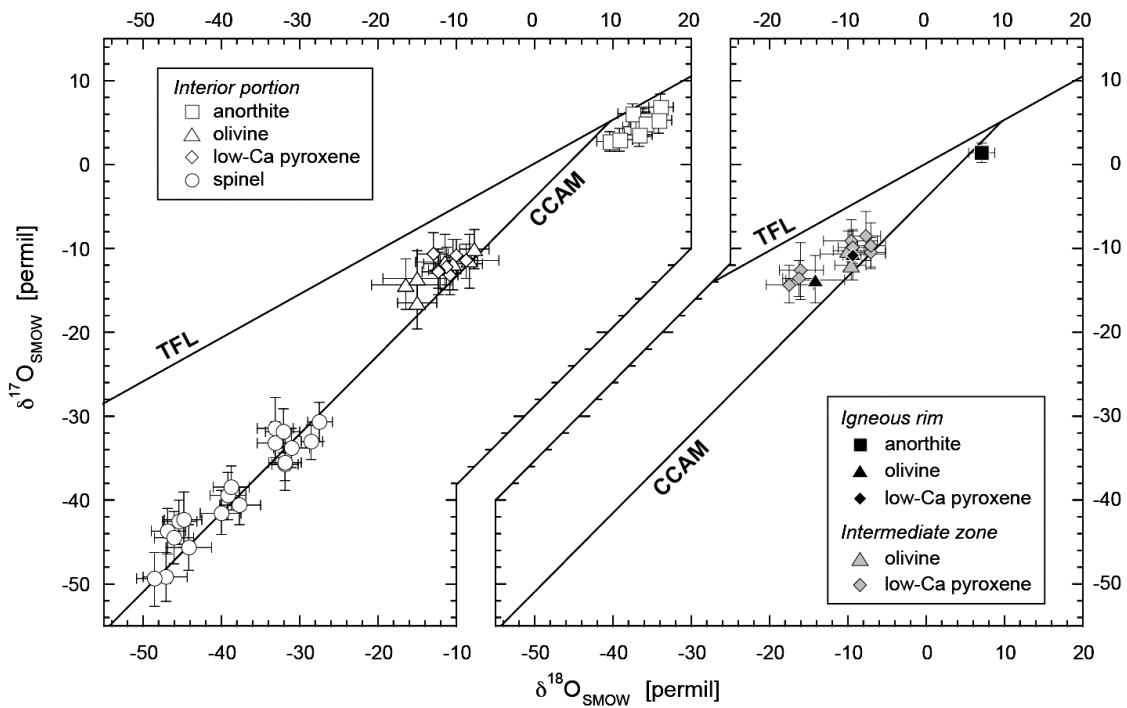
Fig. 8 Oxygen isotopic compositions of minerals in WI-025. The white, black and gray symbols represent the analyses of the interior portion, the igneous rim and the intermediate zone, respectively. The oxygen isotopic composition in WI-025 is heterogeneous among minerals. The oxygen isotopic compositions of the olivines and low-Ca pyroxenes from all three areas are all distributed in a narrow range despite the very different textures observed in these three areas. TFL and CCAM correspond to terrestrial fractionation line and carbonaceous chondrite anhydrous mineral line, respectively.
