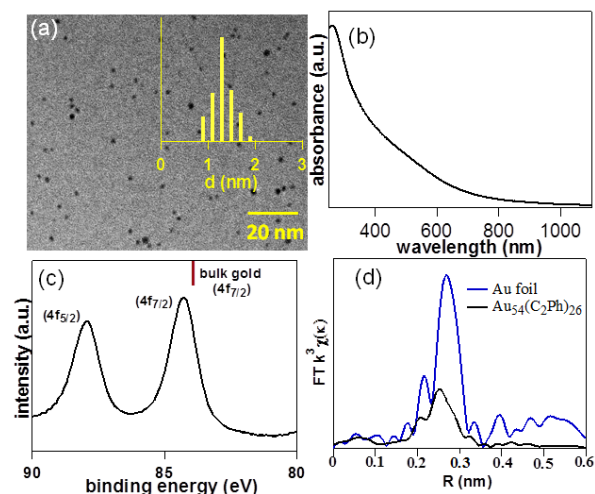
Figure 4. (a) TEM image and size distribution; (b) UV–visible spectrum in chloroform; (c) XP spectrum in the vicinity of Au 4f, (d) Fourier-transform EXAFS spectrum of \text{Au}_{54}(\text{C}_2\text{Ph})_{26} .
