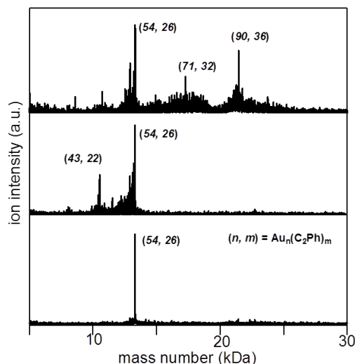
Figure 2. Negative ion MALDI mass spectra of \text{Au:C}_2\text{Ph} produced from 1a (below), 1b (middle), and 1c (above) using chloroform as the extraction solvent.
