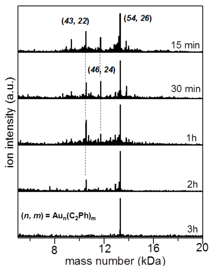
Figure 3. Negative-ion MALDI mass spectra of \text{Au:C}_2\text{Ph} obtained from Au:PVP ( 1a ) for five different reaction times.
