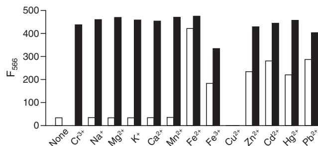
Figure 3. Changes in the fluorescence intensity ( F_{566} ) of BDP-DPA upon the addition of different metal ions. Spectra were acquired in aqueous acetonitrile solution (acetonitrile/water = 9/1, v/v). White bars represent the addition of an excess of the appropriate metal ion (1 mM for \text{Na}^+ , \text{Mg}^{2+} , \text{K}^+ , and \text{Ca}^{2+} . 500 \mu\text{M} for all other ions) to a 1 \mu\text{M} solution of BDP-DPA . Black bars represent the subsequent addition of 500 \mu\text{M} of \text{Cr}^{3+} to the solution. Excitation was provided at 535 nm.
