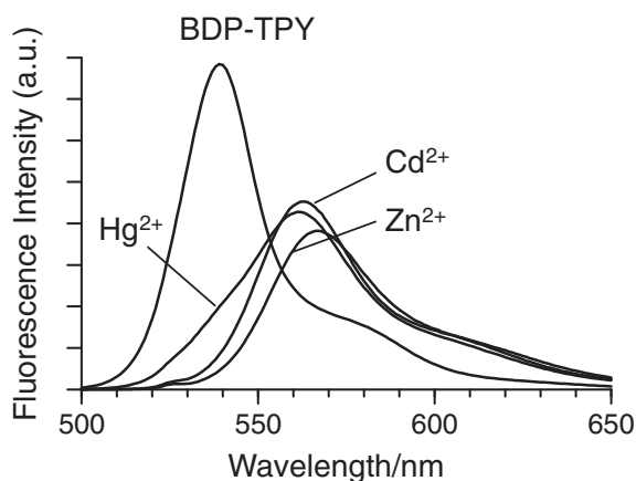
Figure 4. Fluorescence spectra of BDP-TPY in the presence of different metal ions (50 \mu\text{M} ) in aqueous acetonitrile solution (acetonitrile/water = 9/1, v/v) with excitation at 525 nm. The concentration of BDP-TPY was 1 \mu\text{M} .
