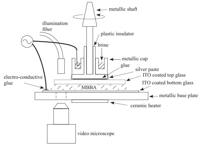
FIG. 1. Schematic diagram of sensor.
