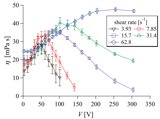
FIG. 3. (Color online) Applied voltage dependence of apparent viscosity for several shear rates. The frequency of the applied electric field is fixed at 60 Hz. For \dot{\gamma} = 3.93, 7.85, 15.7 , and 62.8 \text{ s}^{-1} at the edge r = 30 mm, the rotational speeds of the upper disk are 0.125, 0.25, 0.50, 1.0, and 2.0 rpm, respectively. Since data for \dot{\gamma} = 3.93 \text{ s}^{-1} approach the rheometer’s detection limit, we expect that their values are slightly less than the actual values.
