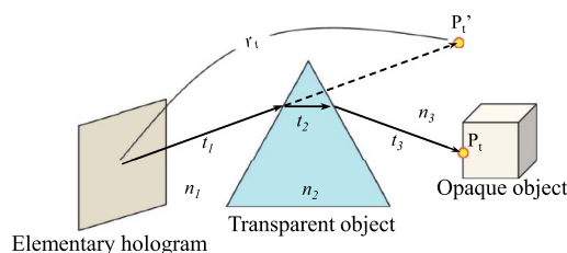
Fig. 10. (Color online) Refraction of the light ray.
