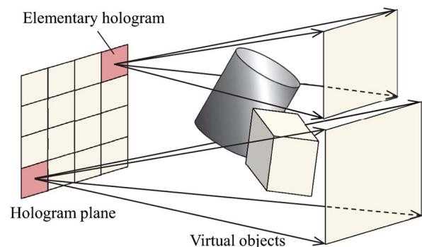
Fig. 2. (Color online) Ray tracing from each elementary hologram.
