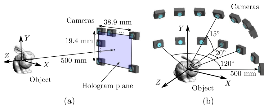
Fig. 6. (Color online) Camera arrangement: (a) for capturing elementary images for experiment I, (b) for SFS.
