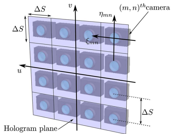
Fig. 3. (Color online) Hologram plane and camera arrangement for calculation of plane hologram.
