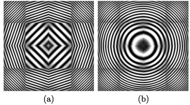
Fig. 2. Zone plates of CGH using MVI: (a) generated by plane wave assumption, (b) generated by spherical wave assumption.
