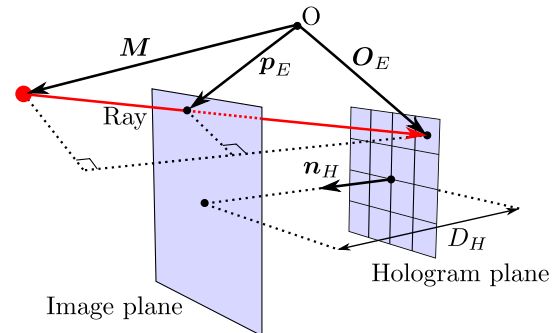
Fig. 5. (Color online) Schematic diagram of volume rendering for proposed method.
