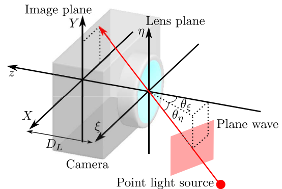
Fig. 1. (Color online) Schematic diagram of camera to capture elementary images.
