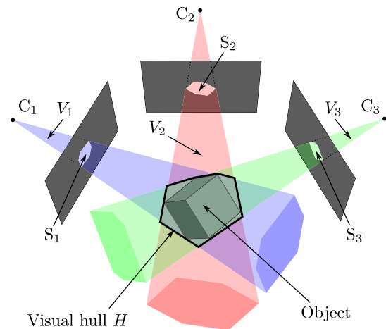
Fig. 4. (Color online) 3D model estimation using SFS.
