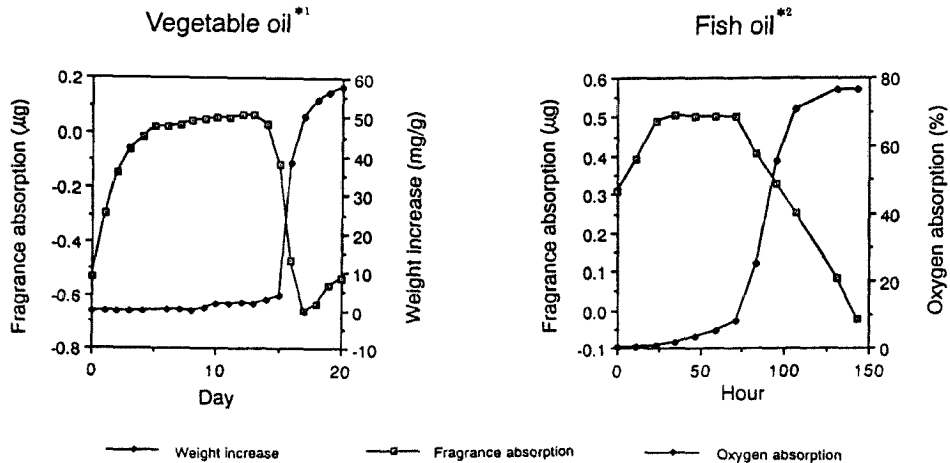
Fig. 1. Changes in fragrance absorption to the synthetic bilayer lipid sensor with respect to weight increase or oxygen absorption of vegetable oil* 1 and fish oil.* 2
