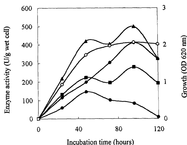
Fig. 1. Alginate degrading enzyme activity and the substrate specificity of intracellular preparation of Alteromonas sp. H-4. Intracellular fraction was prepared at each incubation time of Alteromonas sp. H-4 and its enzyme activity was measured at 30°C for sodium alginate (●), polyM block (◆), polyG block (■) and MG random block (▲) dissolved in 0.1 M Tris-HCl buffer (pH 7.5) as substrate. Growth of the strain was simultaneously measured at absorbance of 620 nm (○).
