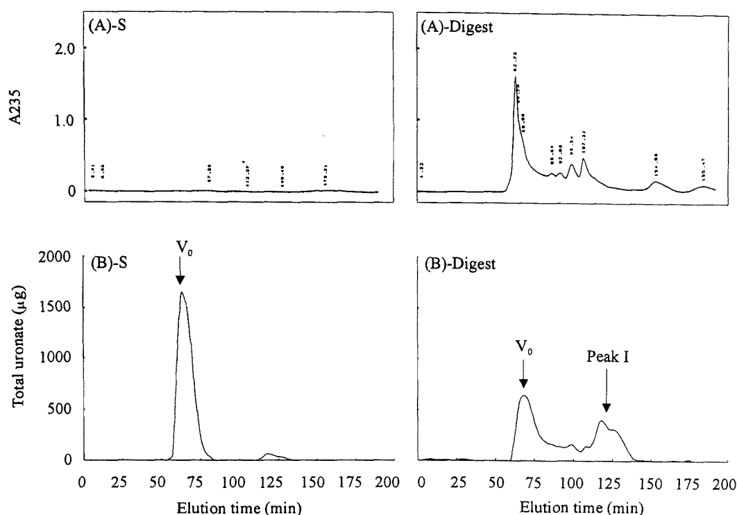
Fig. 4. Elution profiles of the reaction products from polyM block generated by the intracellular polyM specific lyase degradation. Substrate solutions containing 6.5 mg/ml polyM block in 0.1 M Tris-HCl buffer (pH 7.5) were incubated for 24 h at 35°C with the partial purified polyM specific lyase of Alteromonas sp. H-4. The undigested polyM block and reaction mixture was applied to a column (1.34 cm × 40 cm) of Cellulofine GLC 25 m and eluted with 0.1 M Na 2 SO 4 at 28 ml/h. The undigested polyM block ((A)-S) and reaction products ((A)-Digest) were detected at 235 nm using a Hitachi L-4200 UV-VIS detector. The total amounts of uronate of the peaks were determined after separation of undigested polyM block ((B)-S) and reaction products ((B)-Digest) by gel-filtration chromatography. V 0 indicates void volume of the column.
