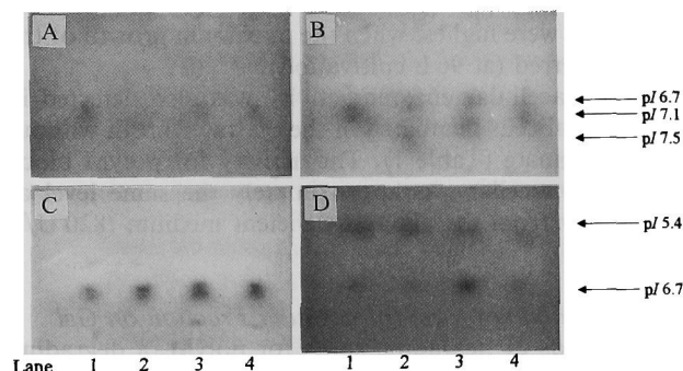
Fig. 2. Activity staining profiles of the intracellular enzymes of Alteromonas sp. H-4 for sodium alginate and homo- and hetero-polymeric blocks after isoelectric focusing gel electrophoresis. (A): sodium alginate, (B): polyG, (C): MG random and (D): polyM blocks. Lane 1: cell-bound activities at 48 h incubation, lane 2: at 72 h incubation, lane 3: at 96 h incubation, lane 4: 120 h incubation.
