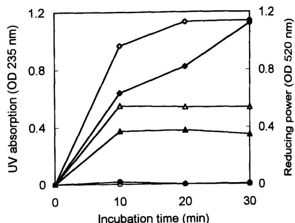
Fig. 3. Measurement of the partially purified intracellular activity for polyM block by UV absorption (open symbol) and reducing power determination (closed symbol). Activity of the partially purified cell-bound enzyme was measured at 30°C for sodium alginate (○ and ●), polyM block (◇ and ◆) and MG random block (△ and ▲) dissolved in 0.1 M Tris-HCl buffer (pH 7.5) as a substrate.
