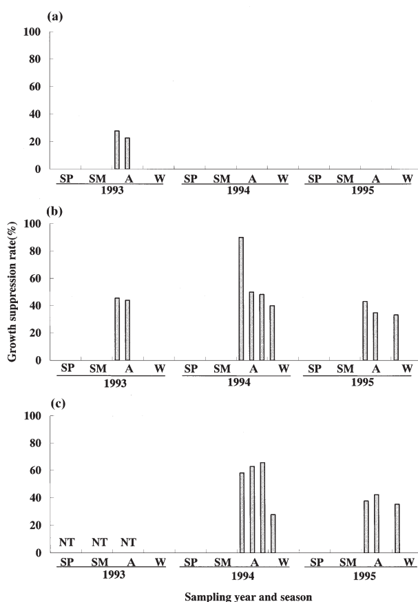
Fig. 1 Seasonal fluctuations of filtratable growth suppression agents for the marine phytoplanktons in the seawater sample collected from the mouth of Funka Bay, Hokkaido, Japan. (a) Tetraselmis sp., (b) Alexandrium catenella , (c) Gymnodinium mikimotoi . SP, spring season March to May; SM, summer season June to August; A, autumn season September to November; W, winter season December to February.
