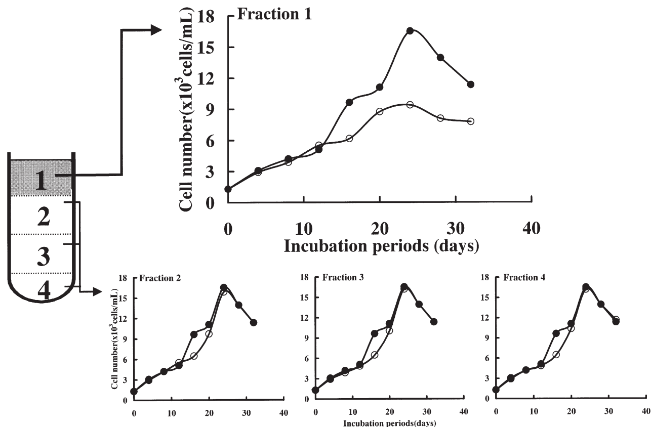
Fig. 3 Growth suppression effect of ultracentrifuged fraction of the culture filtrate of Gymnodinium mikimotoi Ka-34. (●) Control culture inoculated with the filtrated culture of health phytoplankton; (○) experimental culture inoculated with the filtrated culture of the growth suppression against phytoplankton strains.
