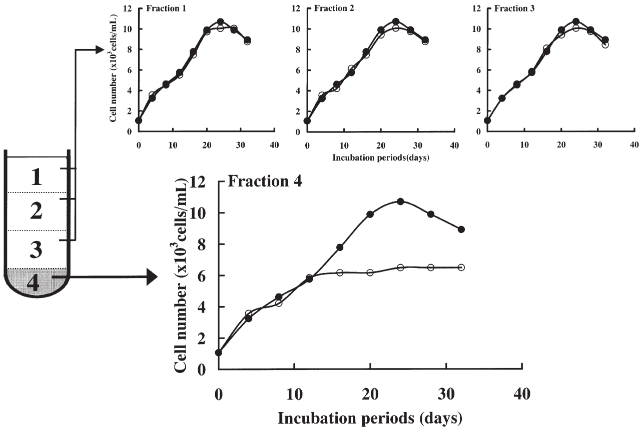
Fig. 2 Growth suppression effect of ultracentrifuged fraction of the culture filtrate of Alexandrium catenella TN-7. (●) Control culture inoculated with the filtrated culture of health phytoplankton; (○) experimental culture inoculated with the filtrated culture of the growth suppression against phytoplankton strains.
