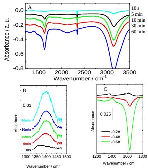
Figure 2. IR spectra at the Pd- V^{++} -Si(111) electrode in a CO_2 saturated 0.1 M Na_2SO_4 solution (A, B) with keeping the potential at -0.7 V for a given period of time under illumination in (A) 1250-3500 cm -1 and (B)
