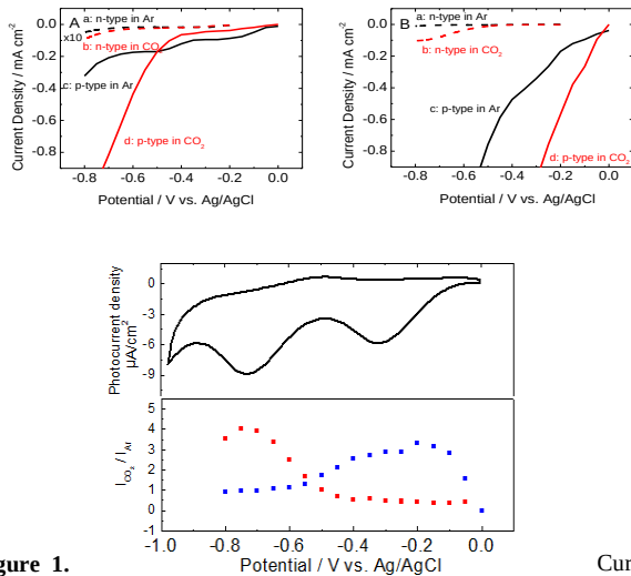
Figure 1. Current-voltage (A) Au- and (B) Pd- V^{++} -Si(111) electrodes in 0.1 M Na_2SO_4 aqueous solutions saturated with Ar (black; a, c) and CO_2 (red; b, d) in dark (n-type, broken line; a, b) and under illumination (p-type, solid line; c, d) with a light intensity of 0.12 mW/cm 2 . Scan rate: 1 mV/s. (C) Top panel: Cyclic voltammogram of p-type V^{++} -Si(111) electrodes in a 0.1 M Na_2SO_4 aqueous solution saturated with Ar under illumination with a light intensity of 0.12 mW/cm 2 . Scan rate: 100 mV/s. Bottom panel: Ratio between currents at Au- (red) and Pd- V^{++} -Si(111) electrodes (blue) in CO_2 saturated solution and that in Ar saturated solution ( I_{CO_2}/I_{Ar} ) as a function of potential.
