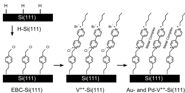
Scheme 1. Schematic illustration of the modification steps of hydrogen terminated (H-) Si(111) surface to obtain Au- and Pd- \text{V}^{++} -Si(111) surfaces. Metal Complex: \text{AuCl}_4^- and \text{PdCl}_4^{2-} . See the text for the detail. 12
