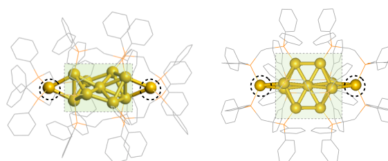
Fig. 1 Side (left) and top (right) views of the crystal structure of [\text{Au}_{11}(\text{Ph}_2\text{P}(\text{CH}_2)_2\text{PPh}_2)_6]^{3+} ( 1 ) representing the [9+2] structure consisting of a \text{Au}_9 core and two gold atoms at the exo positions. The core units and the exo gold atoms are indicated by the shaded rectangles and the dotted circles, respectively.
