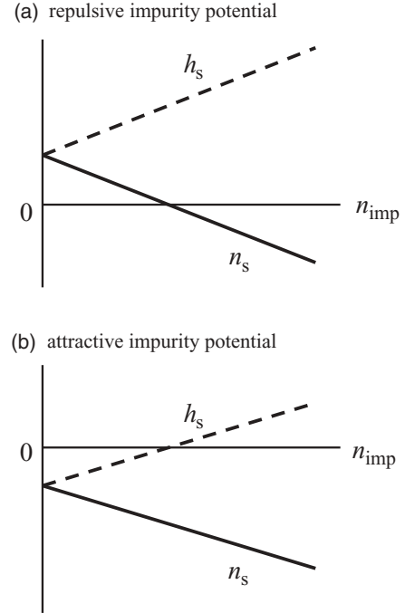
FIG. 1. Normalized spin Nernst coefficient n_s in Eq. (55) and the normalized spin Hall coefficient h_s in Eq. (59) as a function of the impurity density n_{\text{imp}} for (a) a repulsive impurity potential and for (b) an attractive impurity potential.
