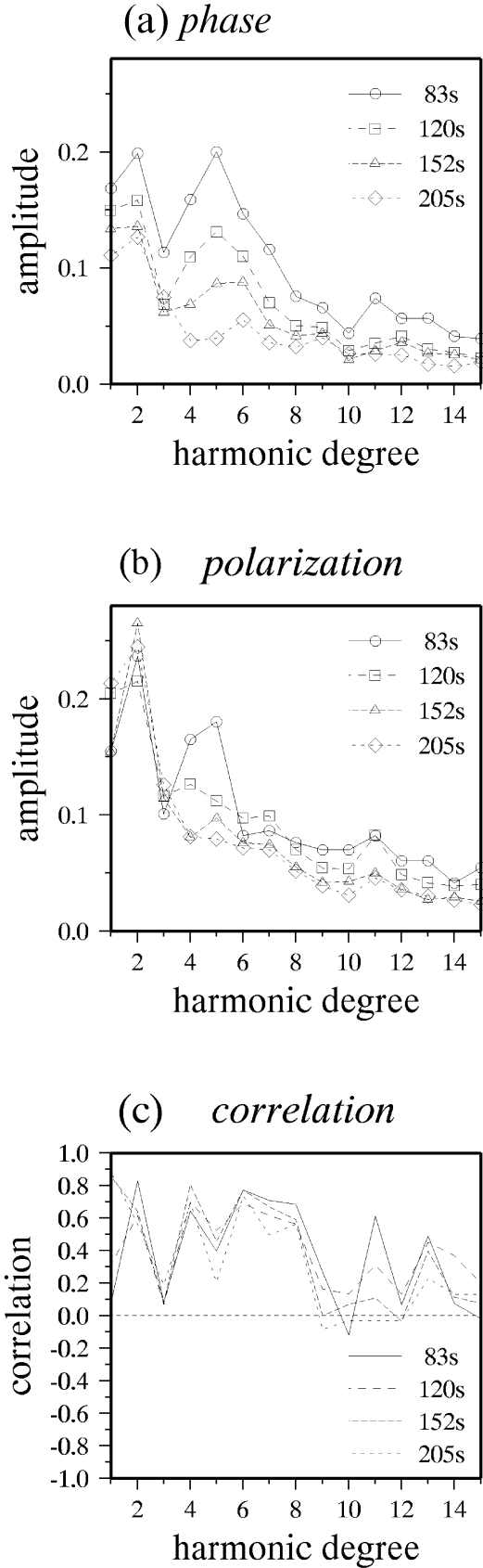
Figure 12. Amplitude spectra of phase velocity maps using (a) phase data and (b) polarization data and (c) their correlation at each period. Circles, squares, triangles and diamonds represent the spectra at 83, 120, 152 and 205 s, respectively.
