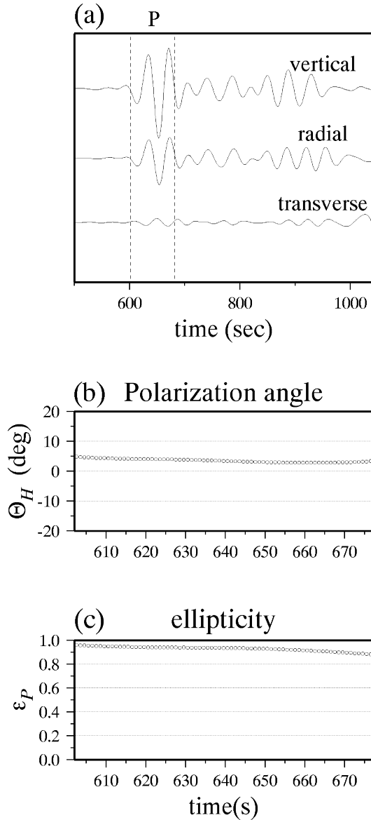
Figure 9. Polarization analysis of lower-mantle P wave recorded at ANMO for an event of 1992 March 2. (a) Three-component seismogram, (b) polarization angles measured clockwise (estimated arrival angle of this seismogram is 3.92 \pm 0.12^\circ ) and (c) ellipticity of polarization ellipse on the horizontal plane plotted as a function of time.
