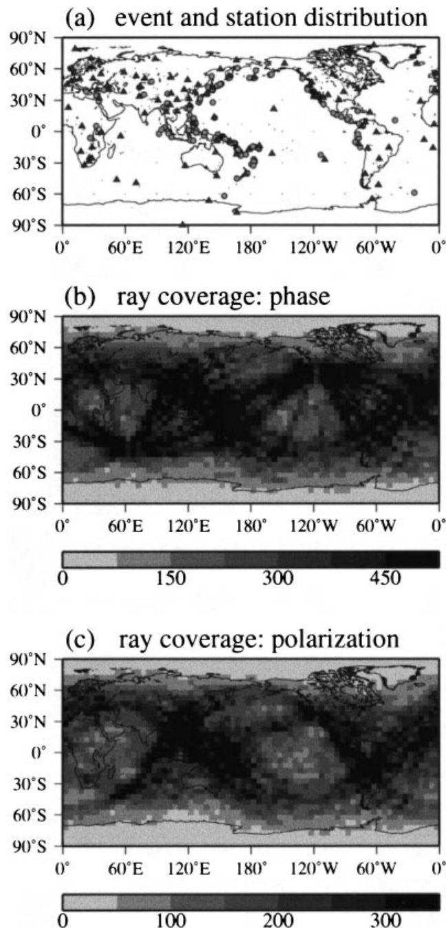
Figure 4. (a) Global distribution of seismic events (circles) from 1990 to 1996 and stations (triangles) used in this study and ray coverage of R1 and R2 for (b) phase data and (c) polarization data at period 152 s. Ray density at each 5^\circ \times 5^\circ grid is calculated by counting points along the great-circle path with an interval of 1^\circ . Note that the contour intervals in (b) and (c) are different.
