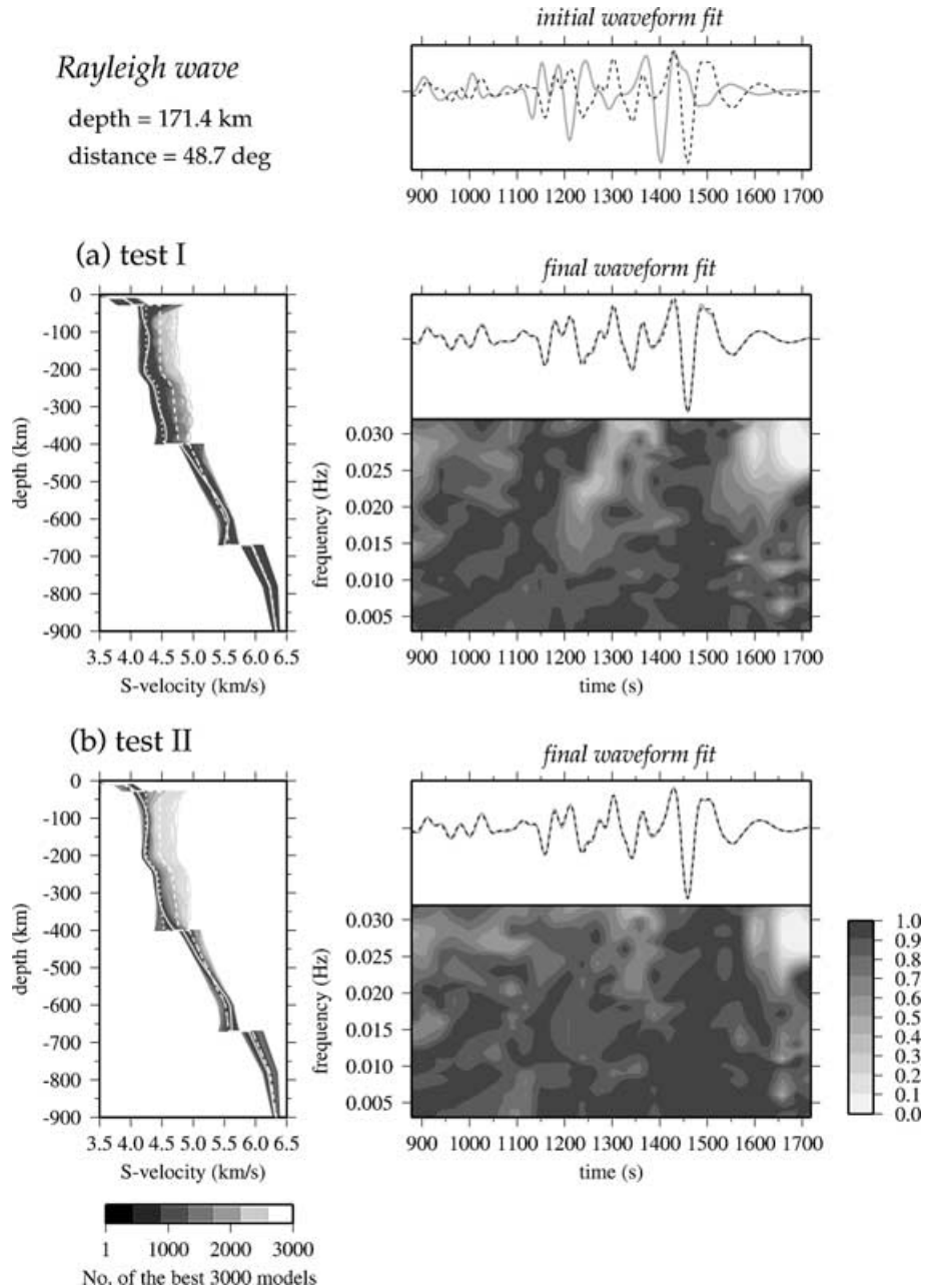
Figure 5. Results of NA inversion for a synthesized Rayleigh wave. Density plots of the 3000 shear wave speed models derived from synthetic tests with a \pm 5 per cent perturbed model are shown in left column. The models are ranked in order of increasing misfit. The best-fitting model is drawn in a solid white line, the reference model in a dashed white line and the true model in a dotted white line. The number of parameters used in test I is 16 ( M_1 = M_4 = 1 , M_2 = 10 and M_3 = 4 ) and in test II is 12 ( M_2 = 6 and others are the same as in test I). The initial and final fits for the waveforms are displayed in the right-hand column together with diagrams of the fit in the F-T domain. Synthetic waveforms for the true model are drawn in a dotted line and for the best-fitting models in a solid grey line.
