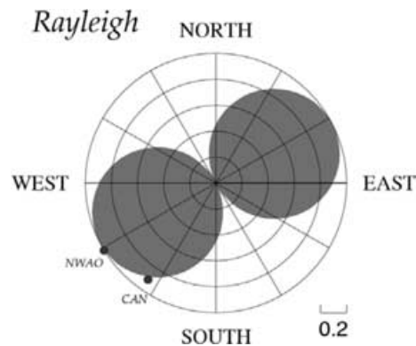
Figure 2. Rayleigh wave radiation pattern for the source parameters used for the calculations of sensitivity kernels. The directions for the two stations, CAN and NWA0, are indicated with dots.
