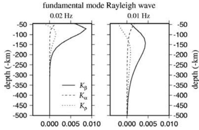
Figure 10. 1-D sensitivity kernels of fundamental mode Rayleigh waves at (left) 0.02 Hz and (right) 0.01 Hz for P - and S -wave speed, and density perturbations.
