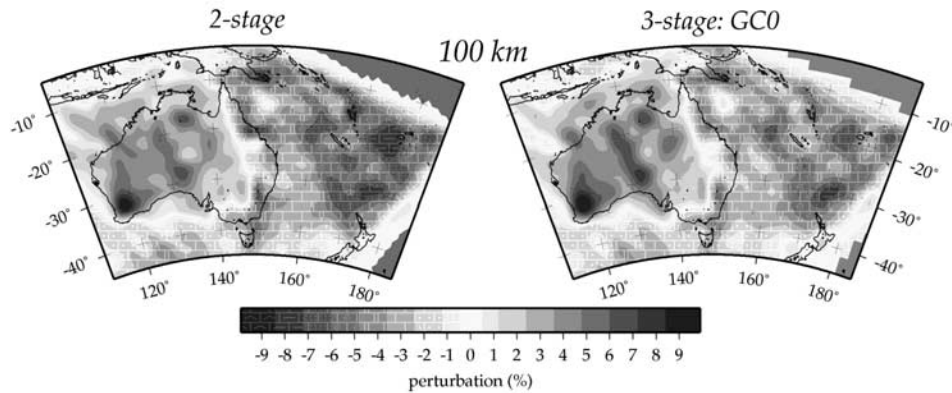
Figure 12. The 3-D shear wave speed models in the Australian region at 100 km depth. (left) Model derived from the two-stage approach and (right) GC0 three-stage model derived from the great circle approximation. The reference wave speed is 4.41 km/s.
