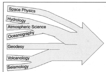
Fig. 1. This schematic shows the possible evolution of the major disciplines currently represented by the International Union of Geodesy and Geophysics. "Geosciences: The Future" recommends organizational changes to accommodate the decreased relevance of disciplinary boundaries. Original color image appears at back of volume.
