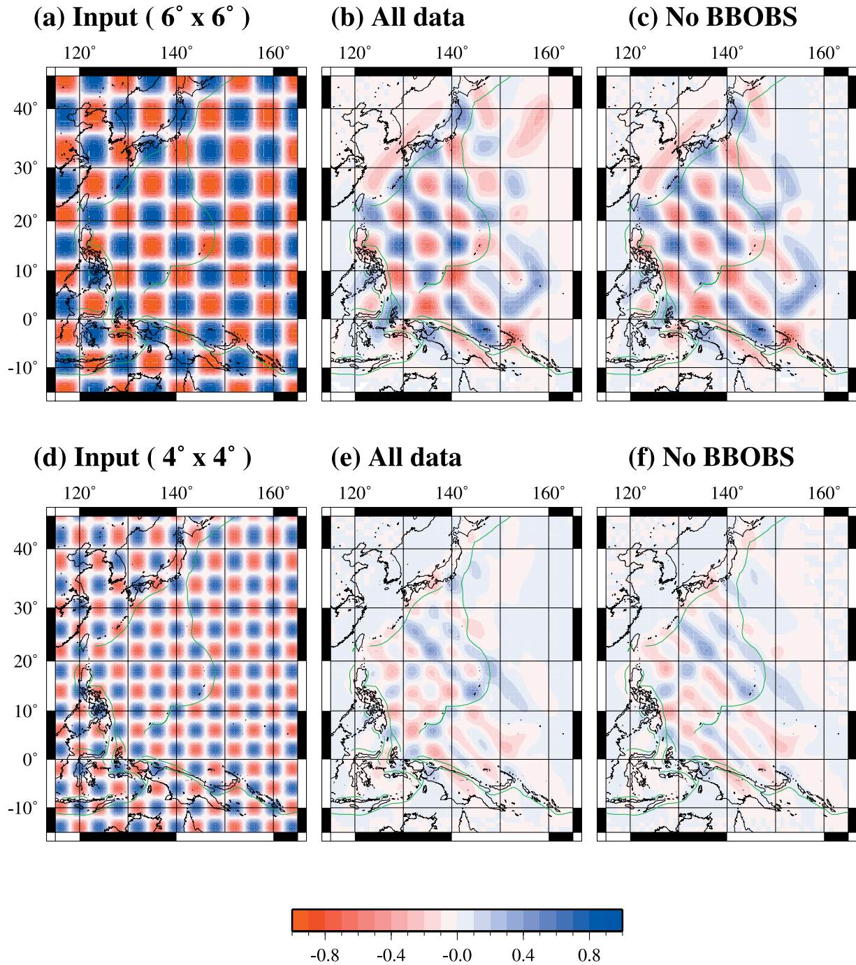
Figure 3. Checkerboard resolution test results for the fundamental mode with different cell sizes: (a–c) 6 \times 6 degrees and (d–f) 4 \times 4 degrees. From the left to right, the input checkerboard models (Figures 3a and 3d), the output models recovered from all the synthetic data (Figures 3b and 3e) and the output models recovered from those without BBOBS data (Figures 3c and 3f).
