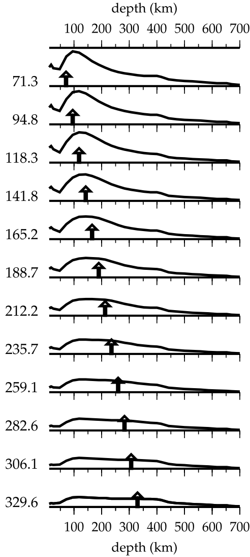
Figure 4. Resolution kernel of the 1-D shear wave speed profile for the site at 18°N and 144°E. The kernel should be delta-like at each depth shown by the arrow if the vertical resolution were perfect.
