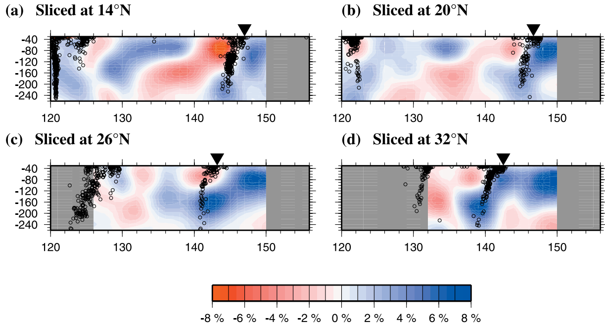
Figure 6. Cross sections of our 3-D shear wave speed model. See Figure 5a for the locations of these cross sections. The subducted Pacific slab can be seen clearly. Inverted triangle on the top of each panel shows the location of the axis of Izu-Bonin-Mariana trench.
