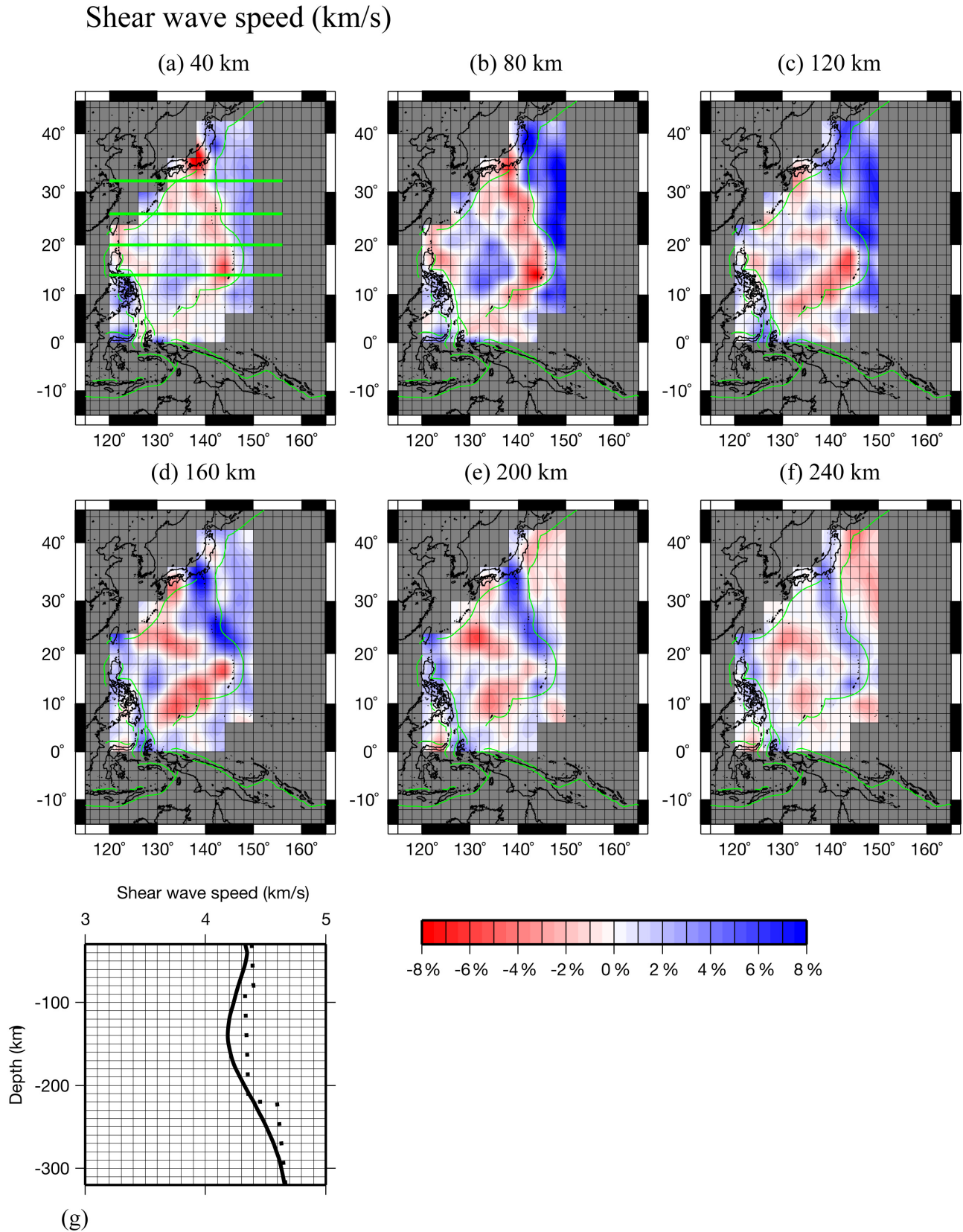
Figure 5. Map projections of the shear wave speed at depths (a) 40, (b) 80, (c) 120, (d) 160, (e) 200, and (f) 240 km. (g) The reference shear wave speed profile (solid line), which is the laterally averaged structure of our 3-D model. The dashed line in Figure 5g is the SV wave speed of PREM at a reference period of 100 s. Green solid lines in Figure 5a show the location of the cross sections given in Figure 6.
