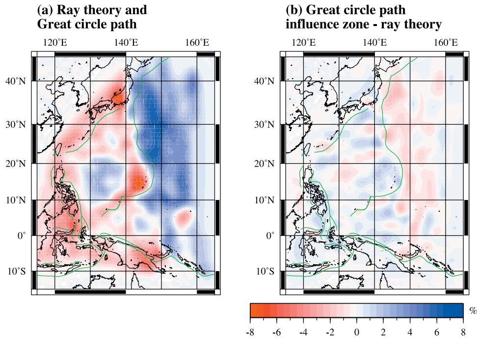
Figure 8. (a) Map projection of the fundamental mode phase speed at a period of 42 s obtained by ray theory with the great circle approximation. (b) Difference in phase speed between the model with the influence zone (Figure 7a) and the model with ray theory Figure 8a.
