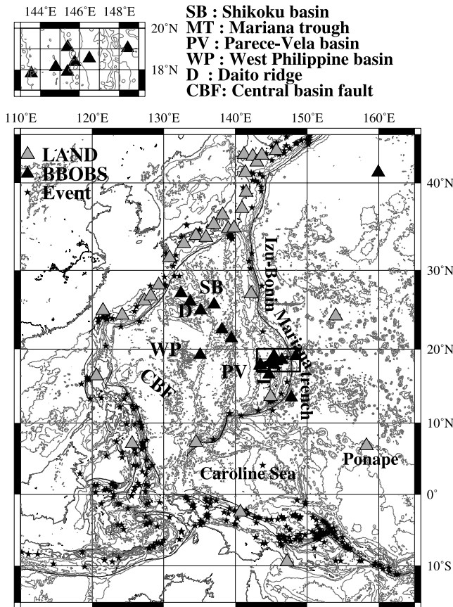
Figure 1. Station and event distributions in the present study. The gray solid triangles are stations on islands, black solid triangles BBOBS stations, and solid stars the event locations. Black square shows the location of a small map at the top. This small map shows the detail of the BBOBS station distribution across the Mariana trough.
