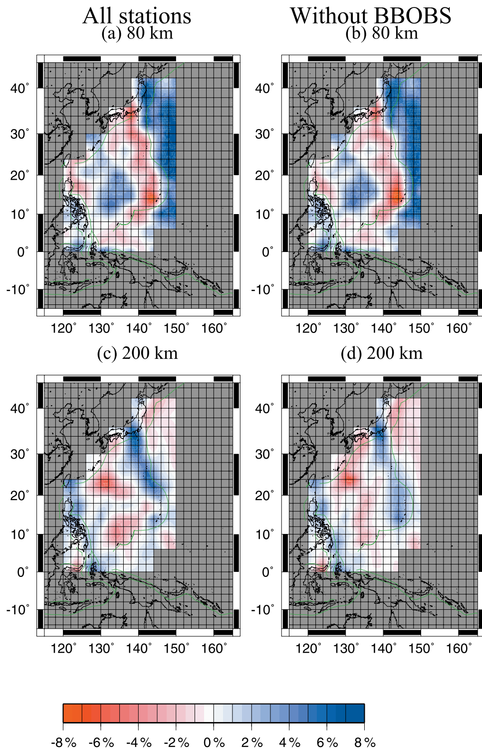
Figure 9. Comparison of the shear wave speed models with and without the BBOBS data. The shear wave speed maps at depths of (a and b) 80 km and (c and d) 200 km are shown. The BBOBS data are used in Figures 9a and 9c and not used in Figures 9b and 9d.
