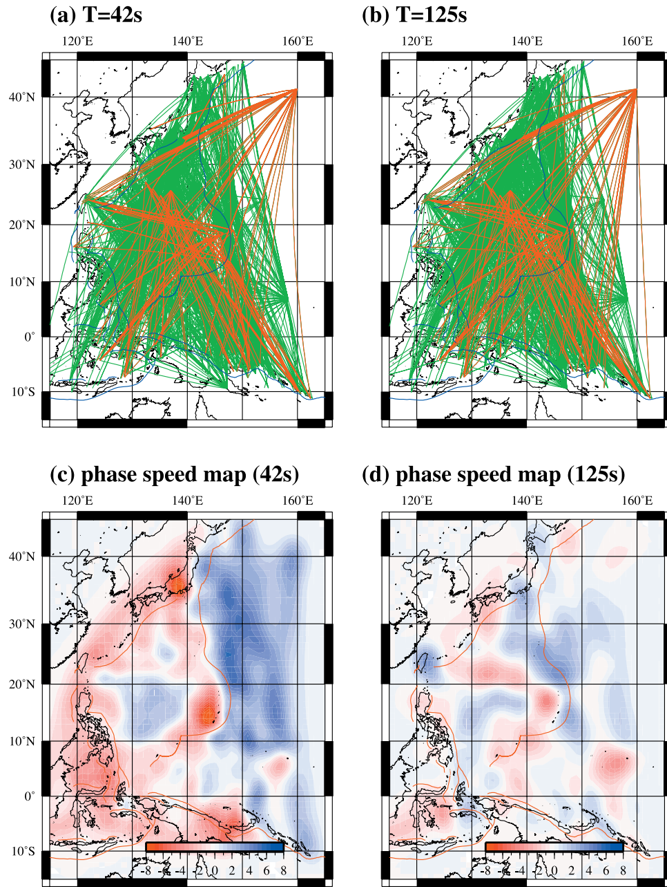
Figure 2. Ray path coverages at (a) 42 and (b) 125 s for the fundamental mode Rayleigh waves. All the rays are traced on the phase speed models at each period, taking the ray bending effect into account. The ray paths to the BBOBS stations are indicated in red. (c) and (d) The corresponding phase speed models, where the reference phase speeds are 3.93 and 4.16 km/s, respectively.
