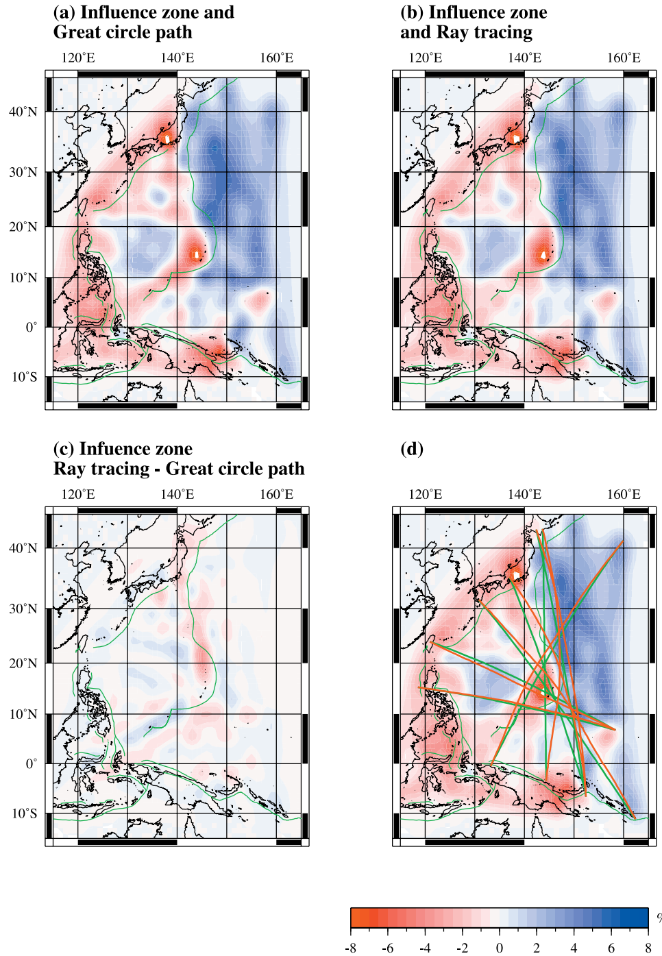
Figure 7. Map projections of the fundamental mode phase speed at a period of 42 s taking into account of the effect of finite frequency via the influence zone around the great circle paths. The effect of ray bending is (a) not taken into account and (b) taken into account. (c) Difference in phase speed between the two models. (d) Examples of the off-great circle paths (red solid lines) and their great circle paths (green thick solid lines). The phase speed map in Figure 7d is the same of that in Figure 7b.
