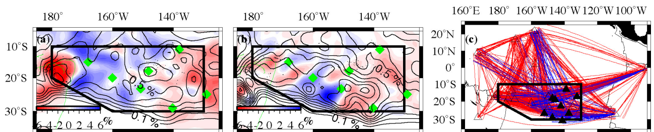
Figure 2. (a, b) Maps of phase speed anomalies and standard errors at periods of 40 and 120 seconds. The average phase speeds are 3.99 and 4.15 km/s, respectively. Green diamonds show the hotspots. Color maps show phase speed and contours show the standard errors with 0.1% interval in each period. (c) Ray distributions we used. Solid and open triangles show the locations of BBOBS and island stations, respectively. Red lines show ray paths along which we measured the phase speeds using only island stations and blue lines using BBOBS stations.
