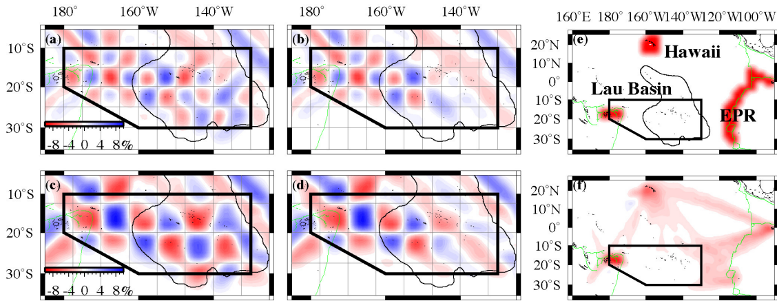
Figure 3. Checkerboard resolution test with (a, b) 5^\circ and (c, d) 7.5^\circ cell at a period of 40 seconds. Figures 3a and 3c show output models recovered by using all data and Figures 3b and 3d show those only by island data. Thin solid black line encircles the superswell region. Thick solid line shows the well-resolved region. The size of the input pattern are shown by grid and amplitude of the input patterns are \pm 10\% . (e) Input slow phase speed anomalies beneath Hawaii, Lau basin and East Pacific Rise. (f) Output model.
