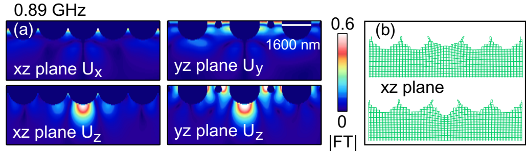
Figure 4. (a) Simulated images of the normalized modulus of the temporal Fourier transform ( |FT| ) of the sample displacement, when excited around a void centre, viewed in cross section at frequency f = 0.89 GHz. The relative magnitudes of the displacements are accurately represented in the set of four plots, which are normalized to a maximum of 1. (b) Deformations at times 1/(2f) ( \pi out of phase) for the xz plane. All cross sections are taken through the centre of a void.
