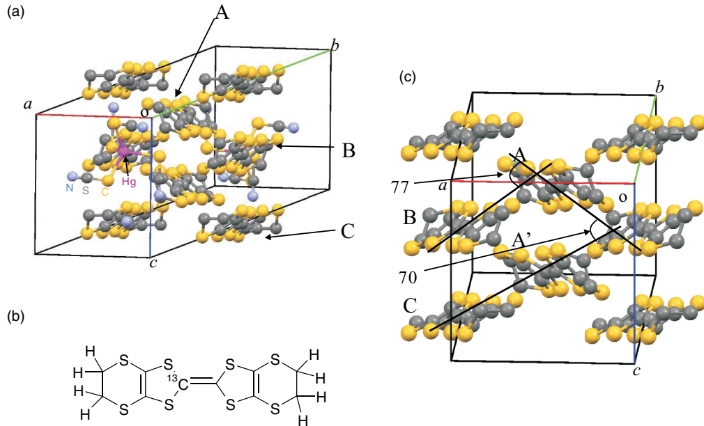
FIG. 1. (Color online) (a) Crystal structure of \alpha -(BEDT-TTF) 2 MHg(SCN) 4 (Ref. 11). (b) Molecular structure of BEDT-TTF- 13 C enriched on one side with 13 C nuclei to prevent the Pake doublet effect. (c) Composite diagram of \alpha -(BEDT-TTF) 2 MHg(SCN) 4 viewed along the b^* axis (Ref. 11). The B and C molecules are located on the inversion center, whereas the A and A' molecules are at general positions and are associated with inversion symmetry.
