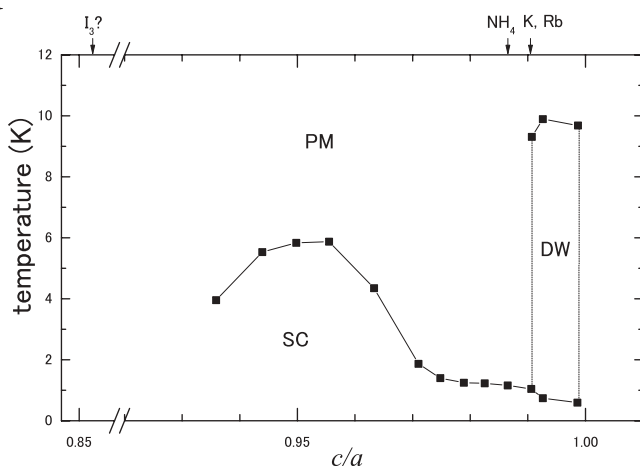
FIG. 2. Phase diagram of \alpha -(BEDT-TTF) 2 X determined by resistance measurement under the uniaxial strain. The horizontal axis is c/a , the ratio of the in-plane lattice constant (Refs. 27 and 28).
