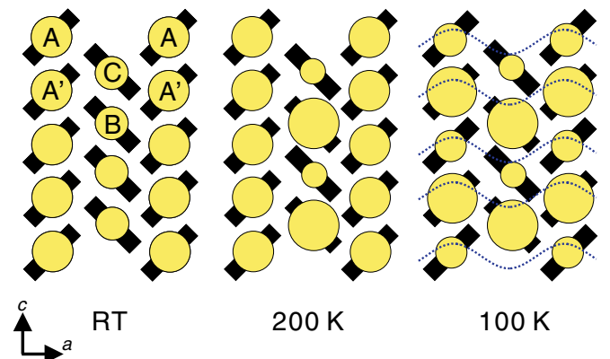
FIG. 5. (Color online) Schematic diagram of the charge disproportionation at typical temperatures. At 100 K, the DW instability was enhanced along the a axis.
