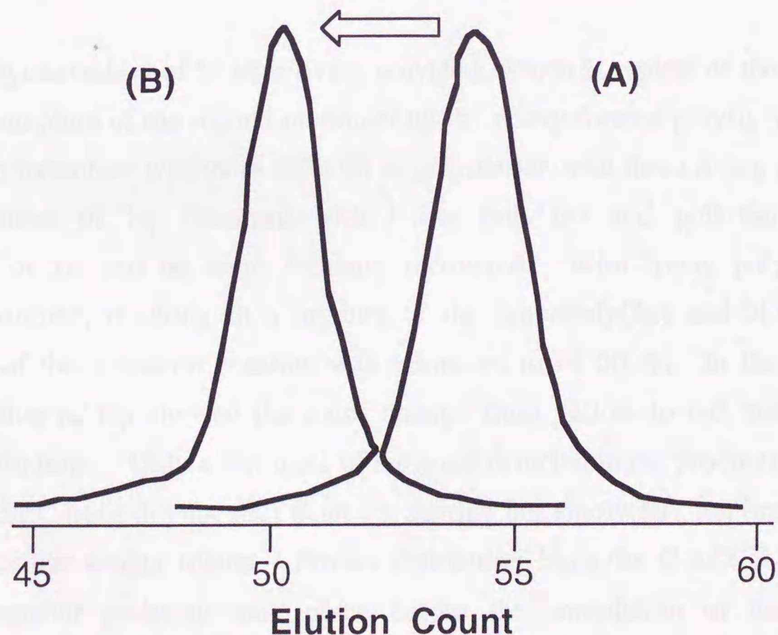
Figure 5-4. SEC curves of polymer 5a at the first-stage polymerization (A) and of poly(2VP- b - 5a - b -2VP) obtained at -78 °C (B) (Table 5-9, run 58): peak A, M_n(\text{obsd}) = 5,800 , M_w/M_n = 1.06 ; peak B, M_n(\text{obsd}) = 15,000 , M_w/M_n = 1.07 (the second monomer was added 0.5 h after the first-stage polymerization).
