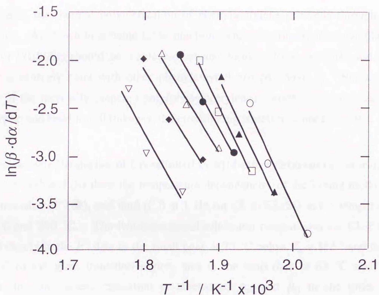
Figure 6-5. The semi-logarithmic plot of \beta (d\alpha/dT) against the inverse of temperature T^{-1} in the IR measurement at heating rate of \beta = dT/dt ( = 3, 5 , and 10^\circ\text{C}\cdot\text{min}^{-1} ). The symbols of ( \circ, \blacktriangle ), ( \square, \bullet, \triangle ) and ( \blacklozenge, \nabla ) denote respectively the slopes at temperatures in the early, intermediate and last stages.
