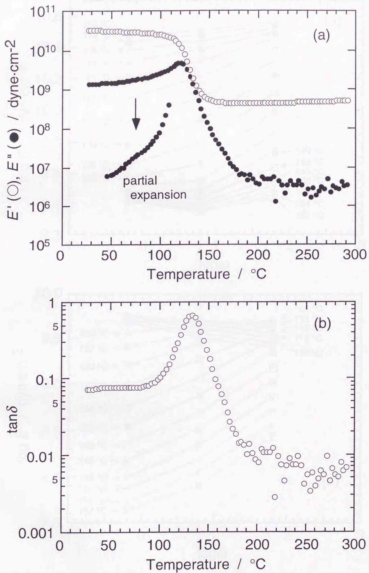
Figure 6-6. The temperature dependencies of the Young modulus E' ( \circ ) and the loss modulus E'' ( \bullet ) (a), and \tan\delta (b) at 1 Hz for CL-P(ES/St) in the temperature region between 0 and 290 ^{\circ}\text{C} .
