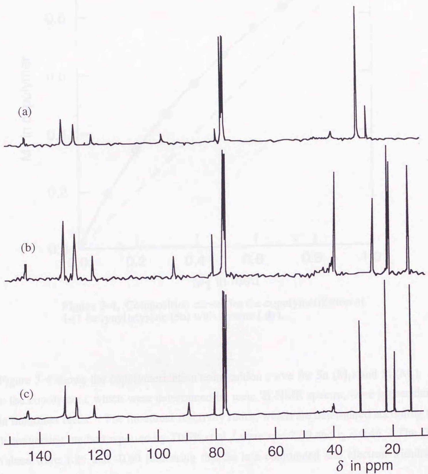
Figure 3-3. ^{13}\text{C} NMR spectra of poly[4-(3,3-dimethyl-1-butynyl)styrene] ( 3a ) (a), poly[4-(3-methyl-1-hexynyl)styrene] ( 4a ) (b), and poly[4-(1-hexynyl)styrene] ( 5a ) (c).
