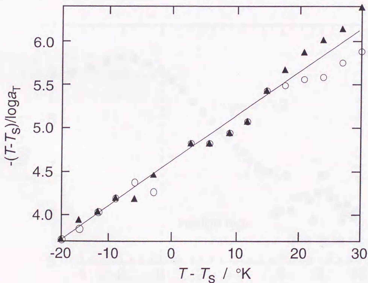
Figure 6-9. The (T-T_s)/\log a_T(T_s) against (T-T_s) plots for the master curves of E' and E'' in CL-P(ES t /St). The symbols of \blacktriangle and \bigcirc denote respectively the values of E' and E'' .
