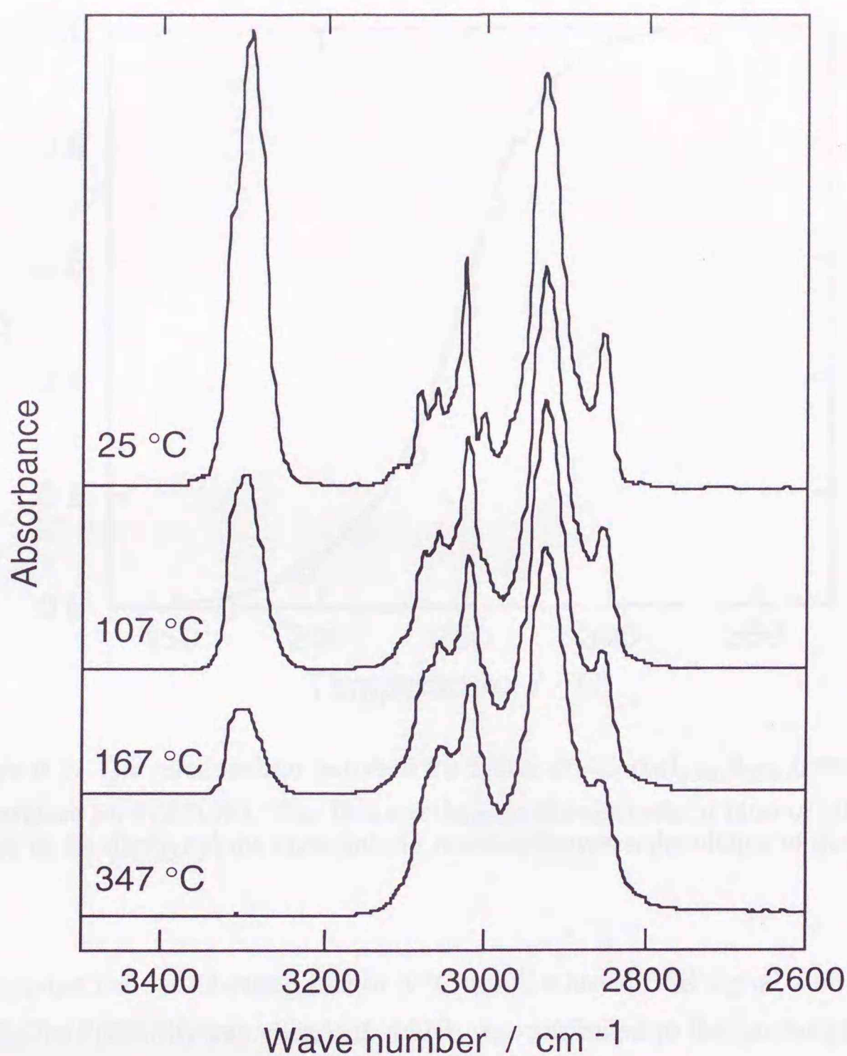
Figure 6-2. The IR spectra of P(ESSt/St) at 25, 107, 167 and 347 °C with the heating of 3 K·min -1 .
