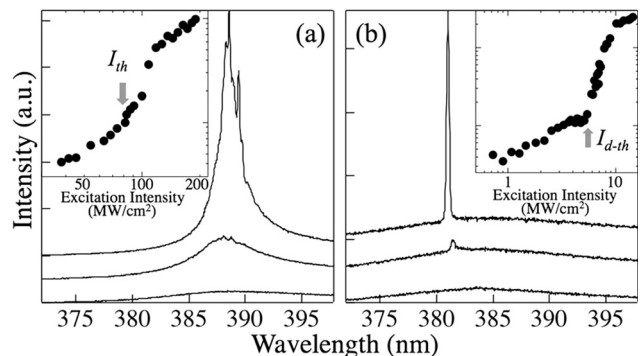
FIG. 2. Emission spectra measured at (a) defect-free and (b) defect sites (arrows 2 and 1 in Fig. 1(d)). The excitation intensities were 0.5, 1.0, and 2.0 times of each threshold from bottom to top. The insets in each figure show the excitation intensity dependences of peak intensities. Arrows indicate the threshold intensities ( I_{th} and I_{d-th} ), respectively.
