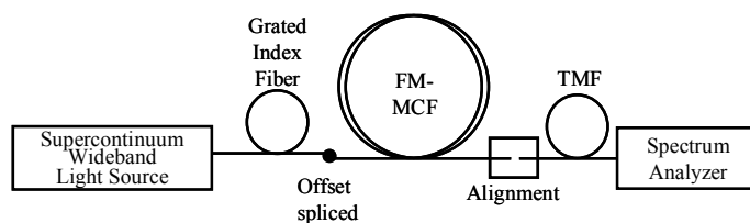
Fig. 10. Measurement setup for measuring wavelength dependence of inter-core crosstalk.
