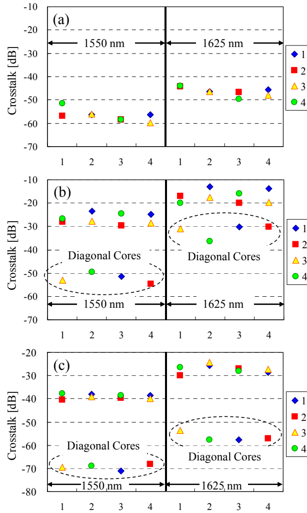
Fig. 7. Results of measured XT_{11-11} of (a) Fiber A, (b) Fiber B and (c) Fiber C.
