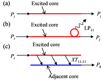
Fig. 6. Measurement procedure of XT_{11-11} .
