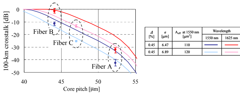
Fig. 8. The comparison of 100-km crosstalk estimation from measured results and simulation results as a function of core pitch.
