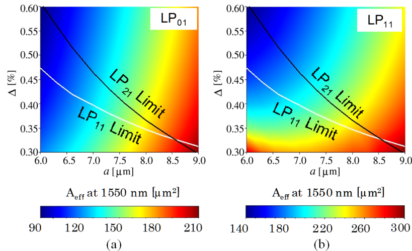
Fig. 1. Structural parameter dependence of A_{\text{eff}} of (a) LP_{01} mode and (b) LP_{11} mode.
