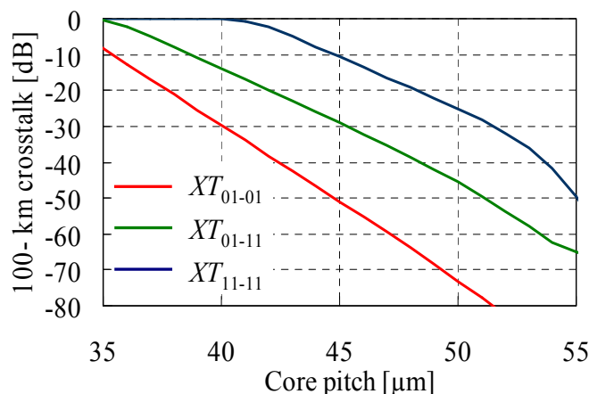
Fig. 2. Simulated inter-core 100-km crosstalk as a function of core pitch assuming a = 6.47 \mu\text{m} and A = 0.45\% .
