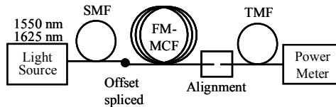
Fig. 5. Measurement system of higher mode crosstalk.
