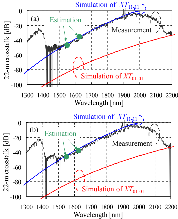
Fig. 9. Wavelength dependence of inter-core crosstalk (a) from core 1 to core 2 and (b) from core 1 to core 4.
