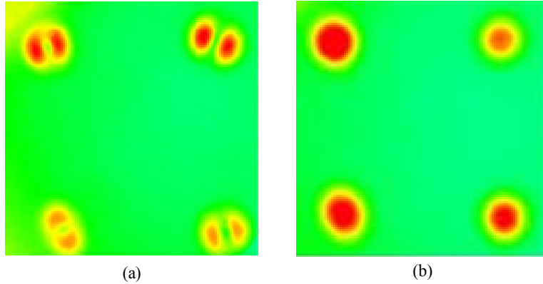
Fig. 4. The NFP at 1550 nm of Fiber B (a) without bends and (b) with bends.
