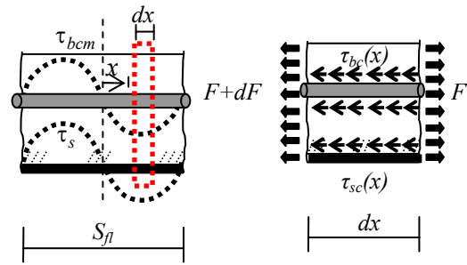
a. Bond stress distribution b. Free body diagram
